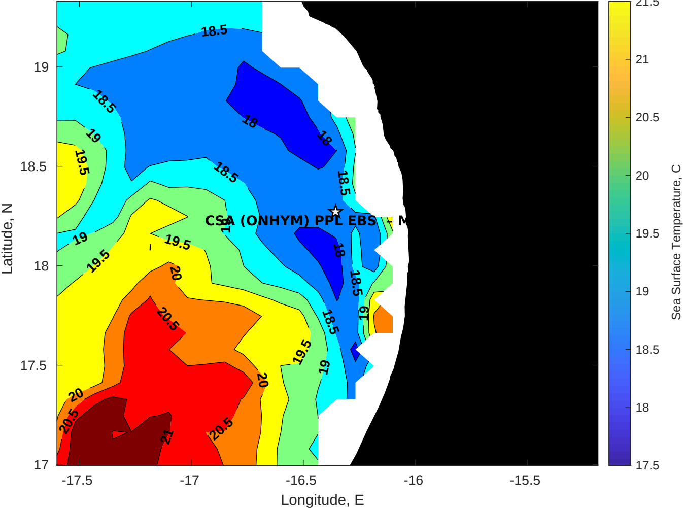
SST for CSA (ONHYM) PPL EBS - Mauritania at 04-May-2025 00:00:00
