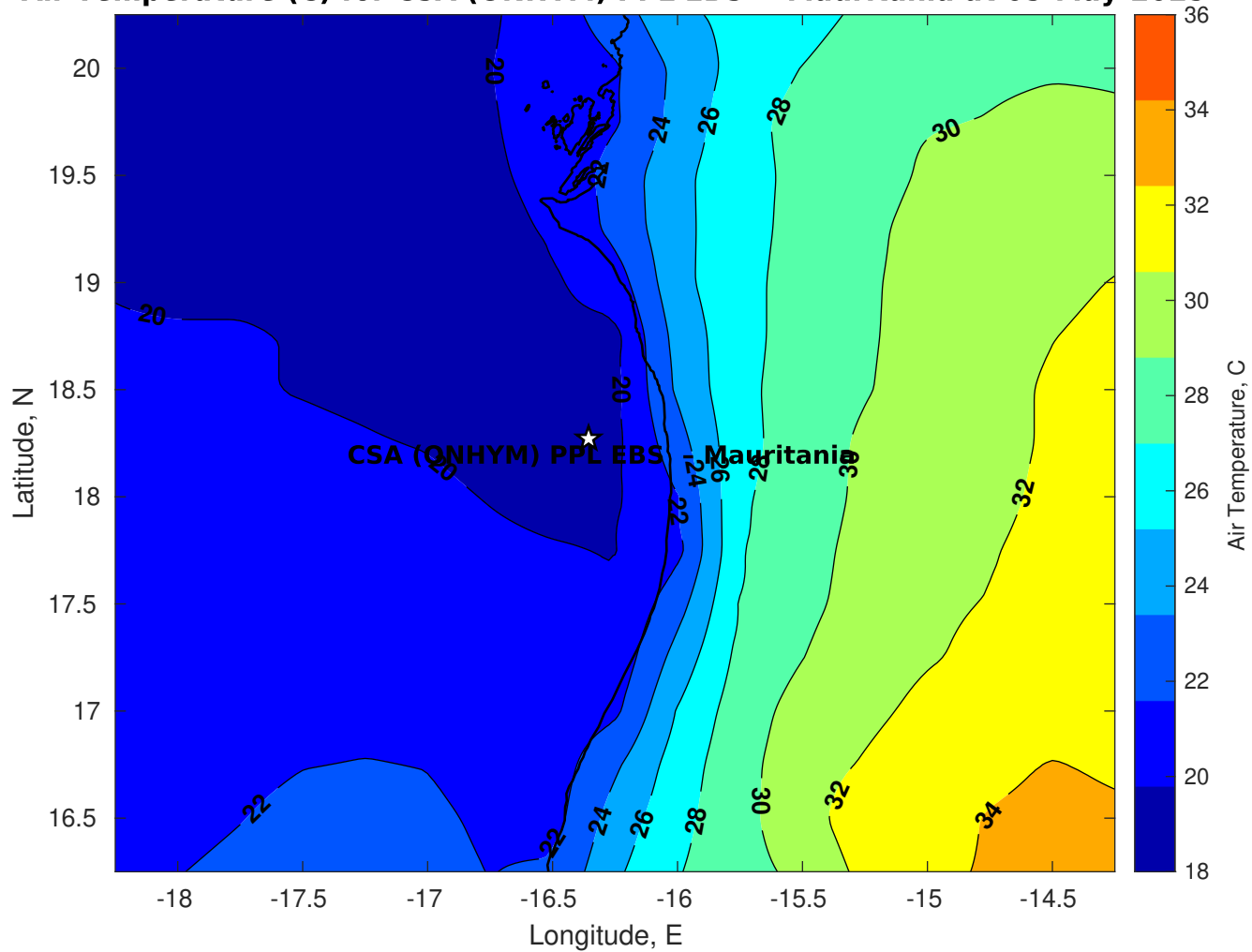
Air Temperature (C) for CSA (ONHYM) PPL EBS - Mauritania at 05-May-2025
