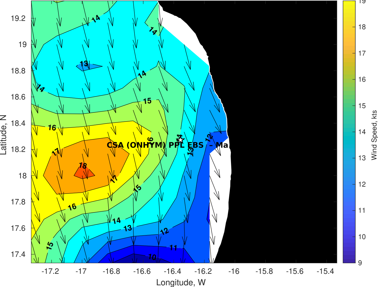
Winds (kts) for CSA (ONHYM) PPL EBS - Mauritania at 05-May-2025 09:00:00
