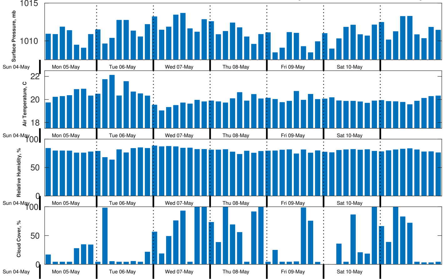
Met Forecast for CSA (ONHYM) PPL EBS - Mauritania from 05-May-2025 00:00:00 to 12-May-2025 00:00:00
