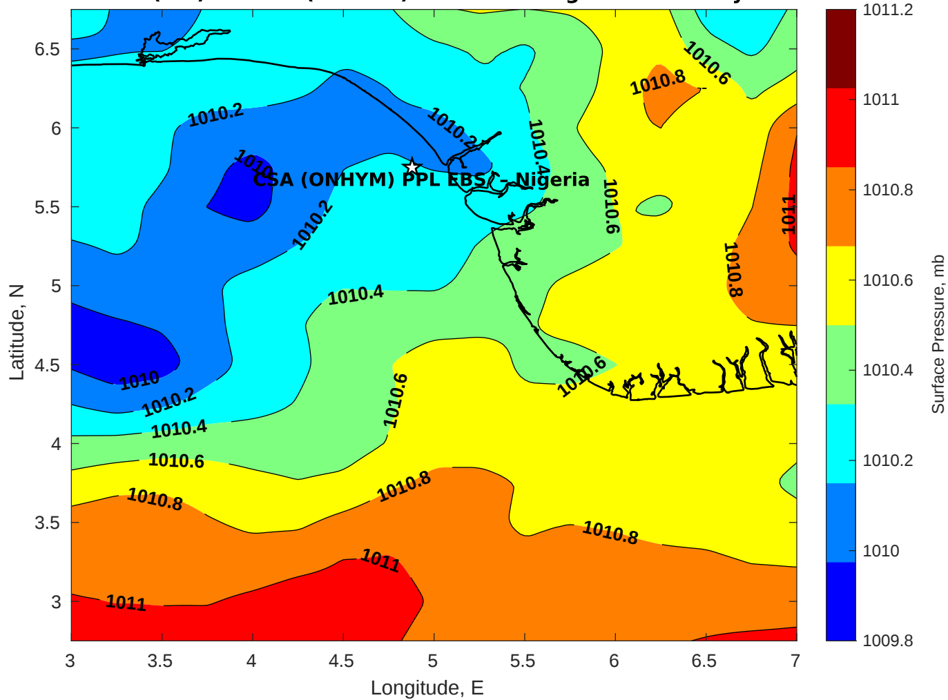
Surface Pressure (mb) for CSA (ONHYM) PPL EBS - Nigeria at 06-May-2025 00:00:00
