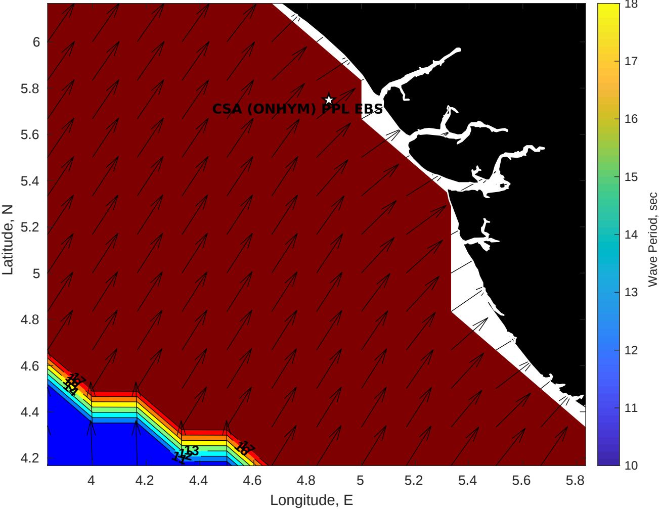
Wave Period (sec) for CSA (ONHYM) PPL EBS - Nigeria at 05-May-2025 09:00:00
