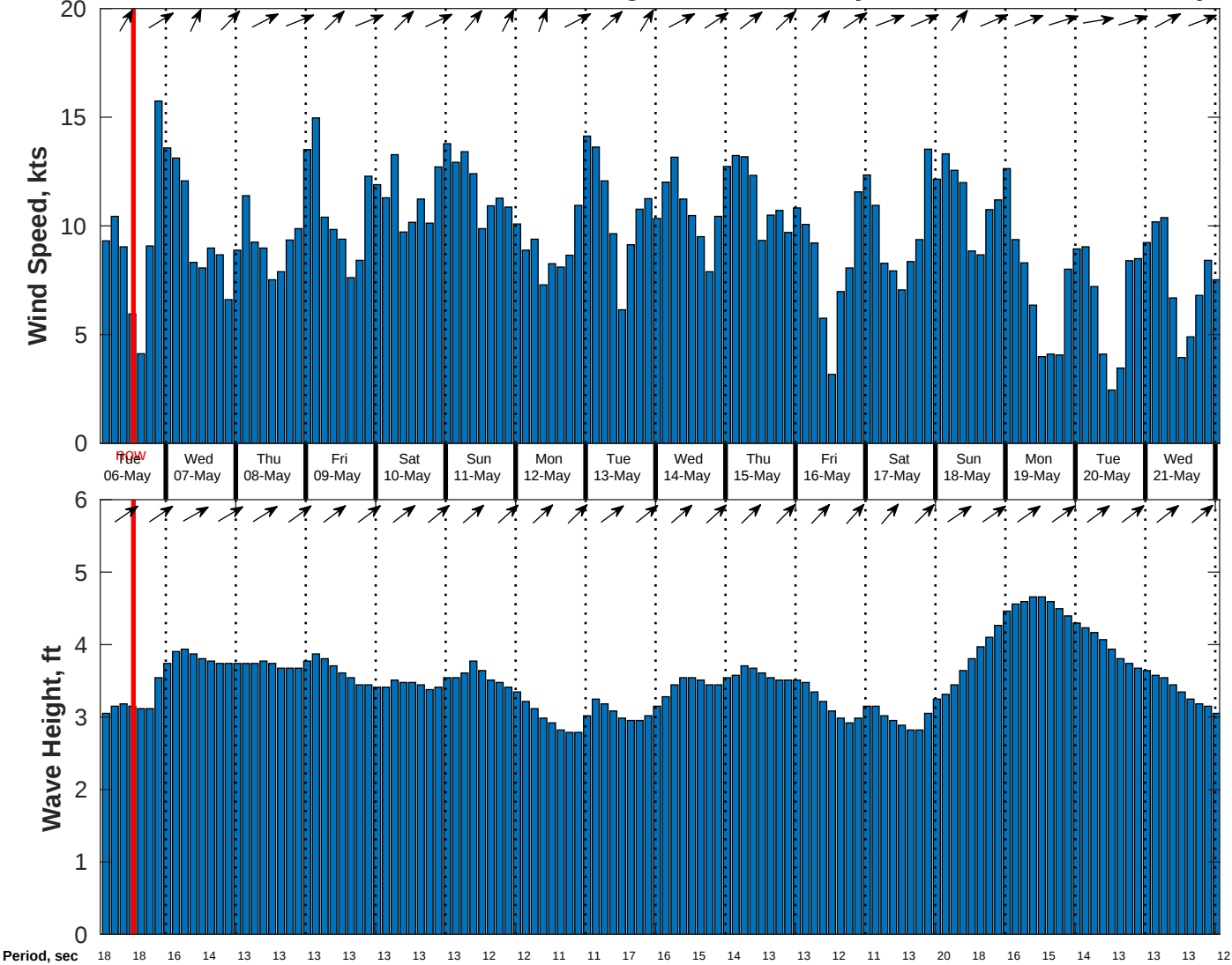
Wind & Wave Forecast for CSA (ONHYM) PPL EBS - Nigeria from 05-May-2025 02:00:00 to 21-May-2025 02:00:00
