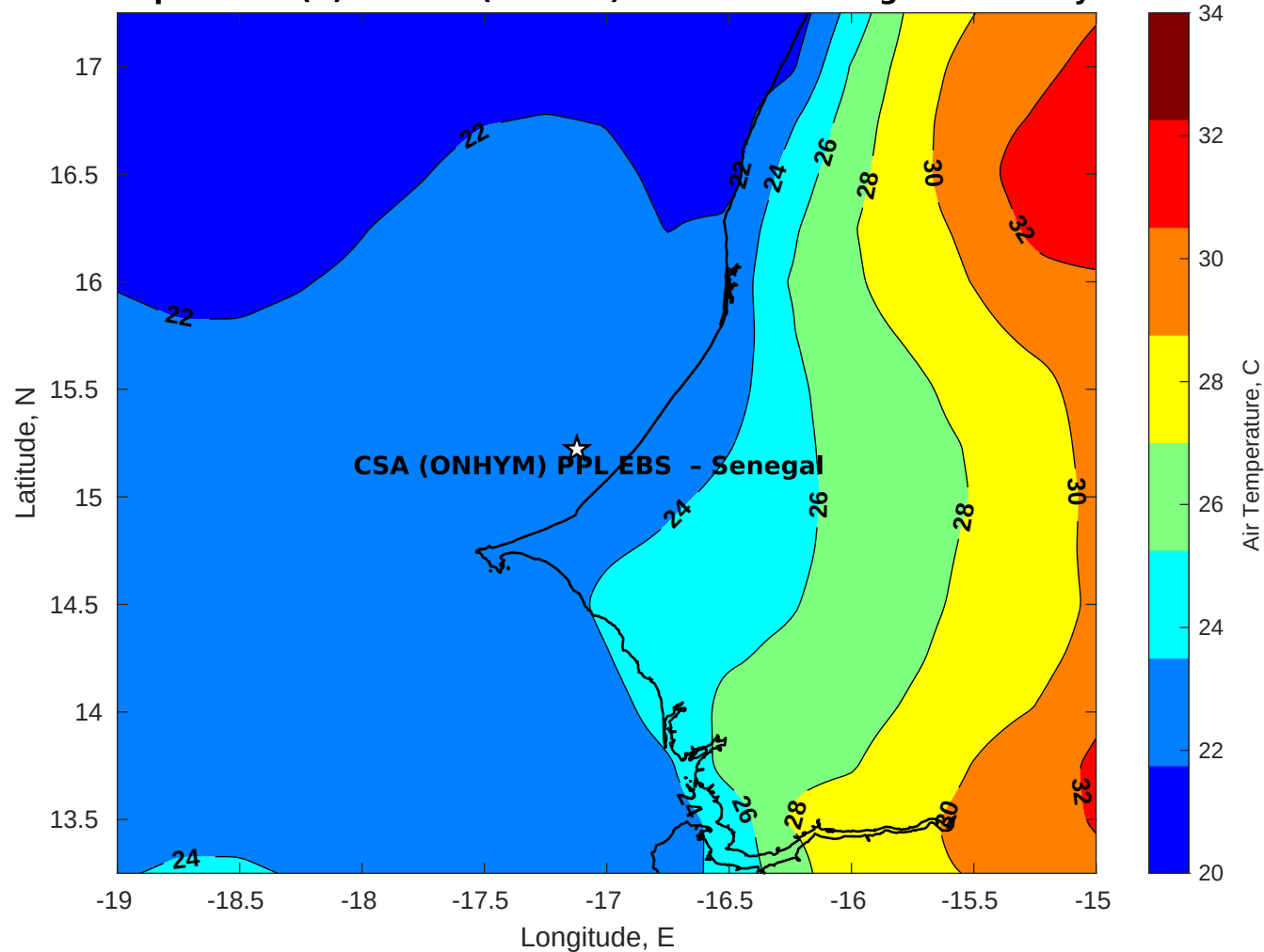
Air Temperature (C) for CSA (ONHYM) PPL EBS - Senegal at 05-May-2025
