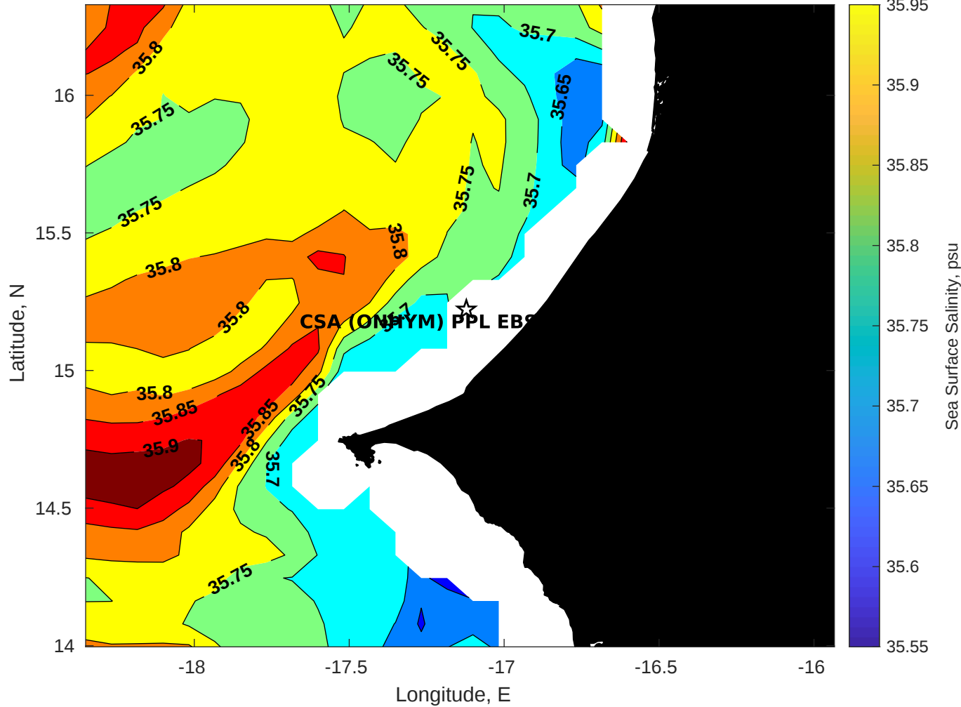
Surface Salinity for CSA (ONHYM) PPL EBS - Senegal at 04-May-2025 00:00:00
