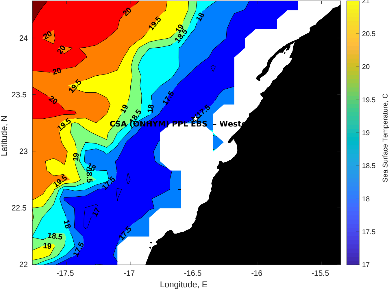
SST for CSA (ONHYM) PPL EBS - Western Sahara at 04-May-2025 00:00:00
