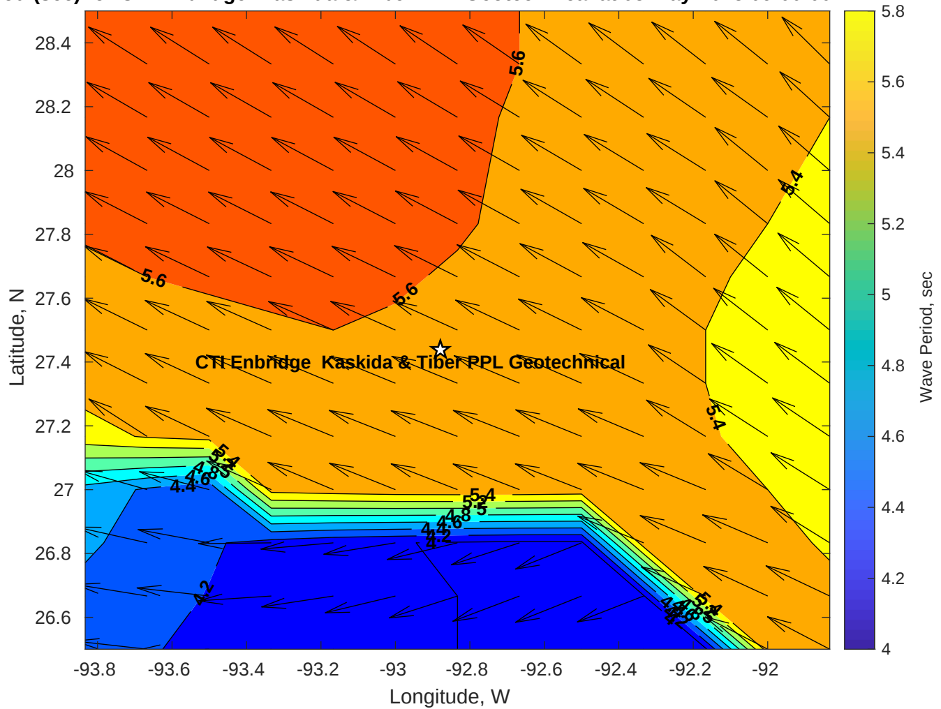
Wave Period (sec) for CTI Enbridge Kaskida & Tiber PPL Geotechnical at 05-May-2025 09:00:00
