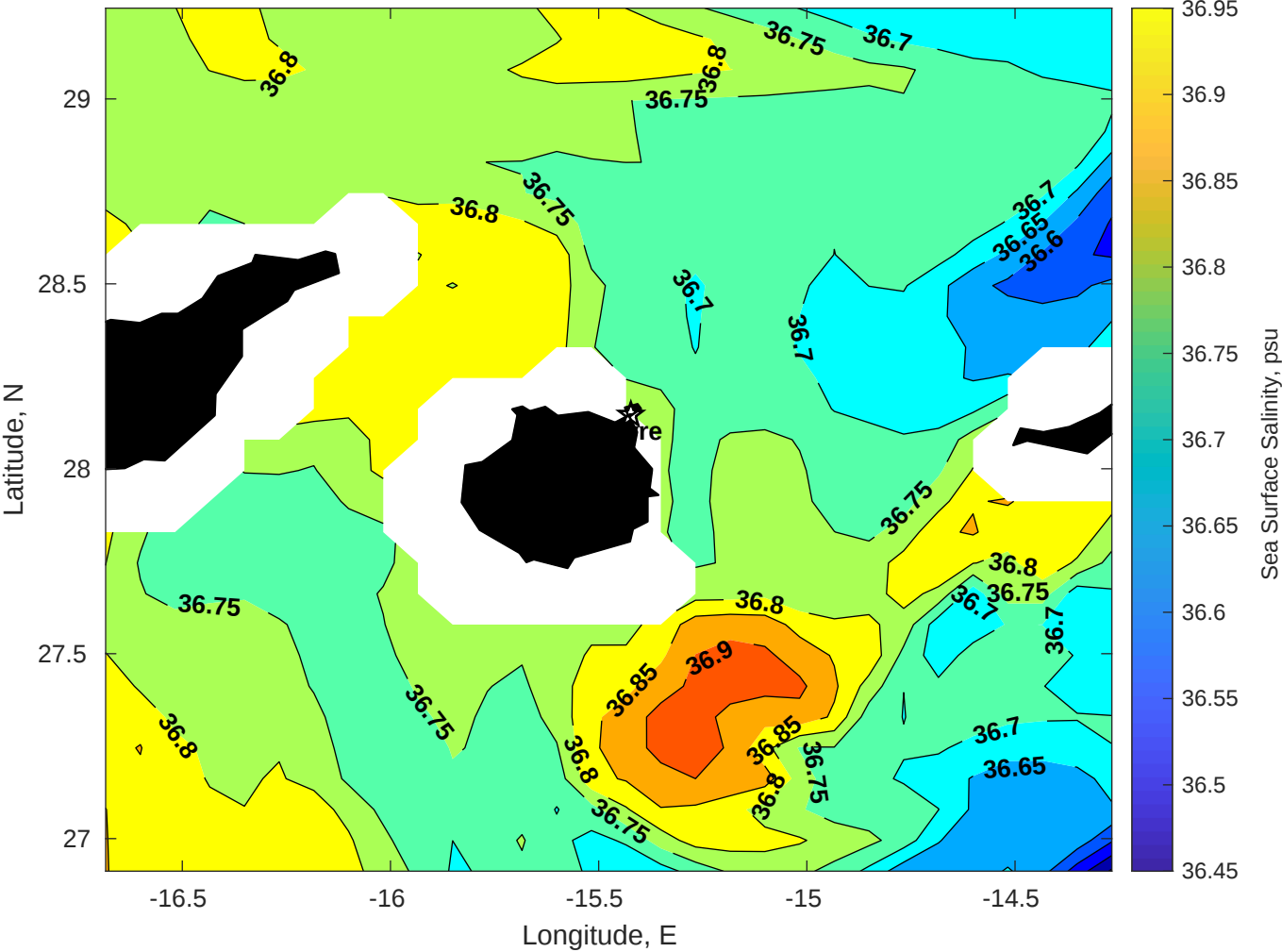
Surface Salinity for Gyre at 04-May-2025 00:00:00
