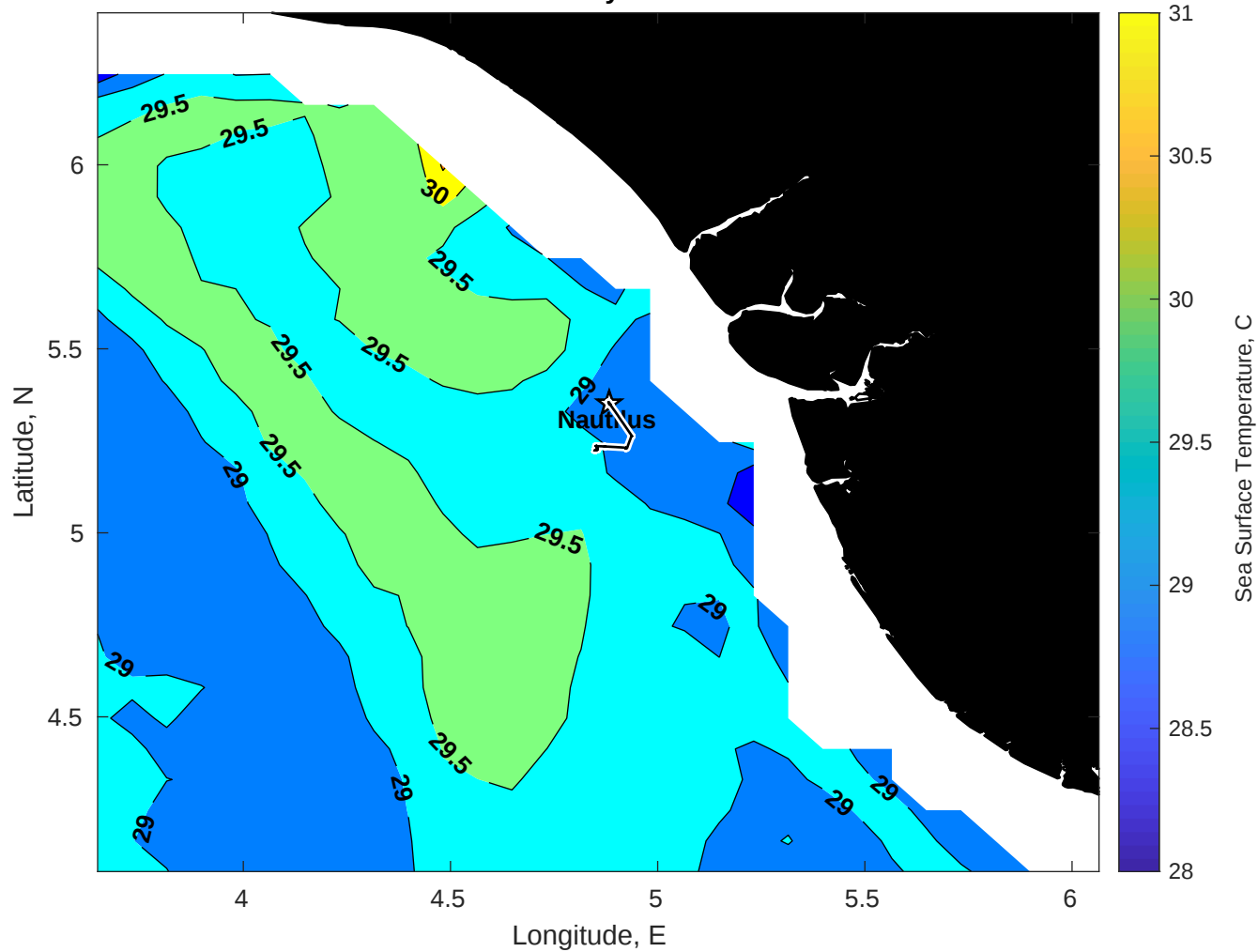
SST for Nautilus at 04-May-2025 00:00:00
