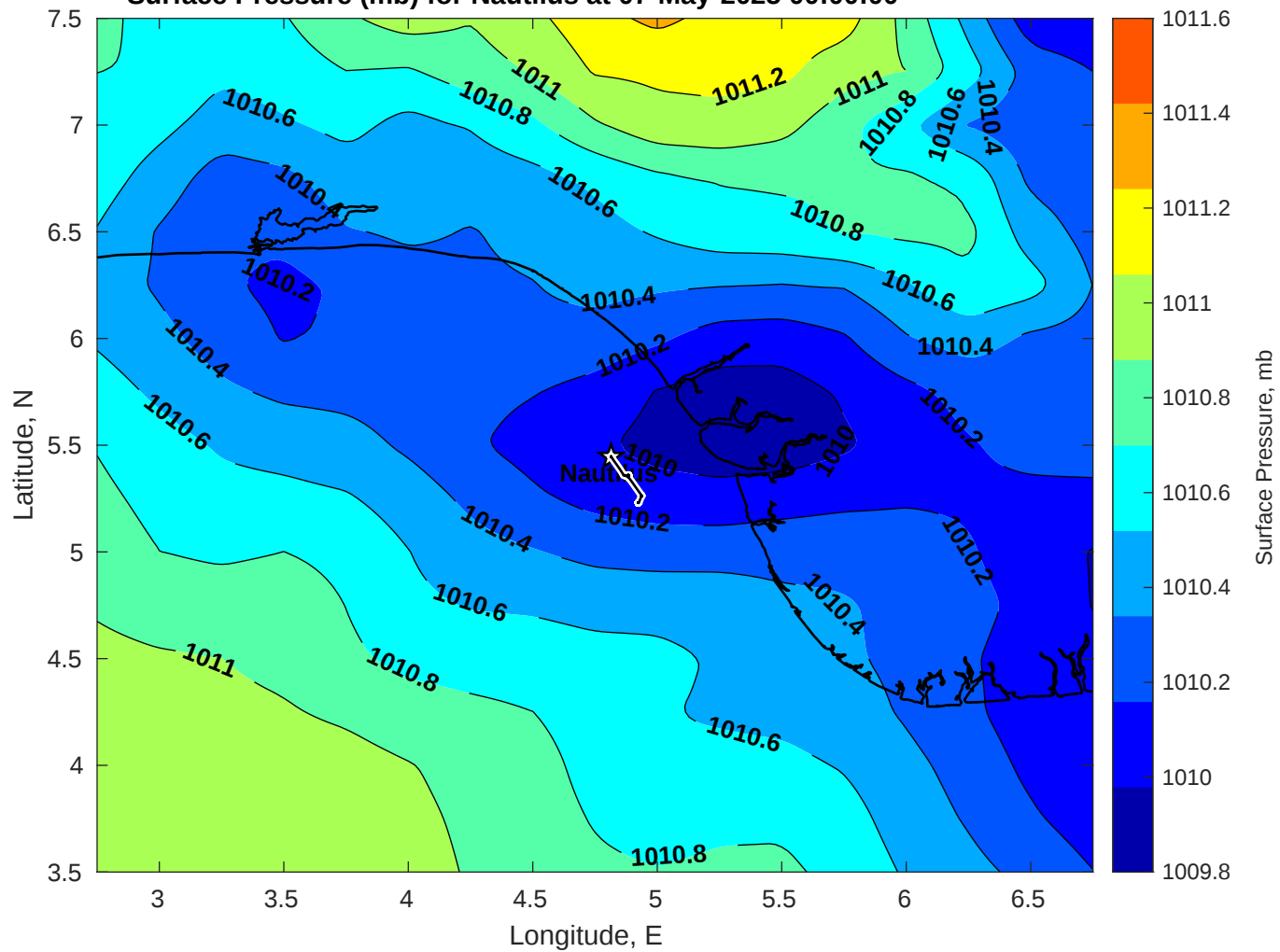
Surface Pressure (mb) for Nautilus at 07-May-2025 00:00:00
