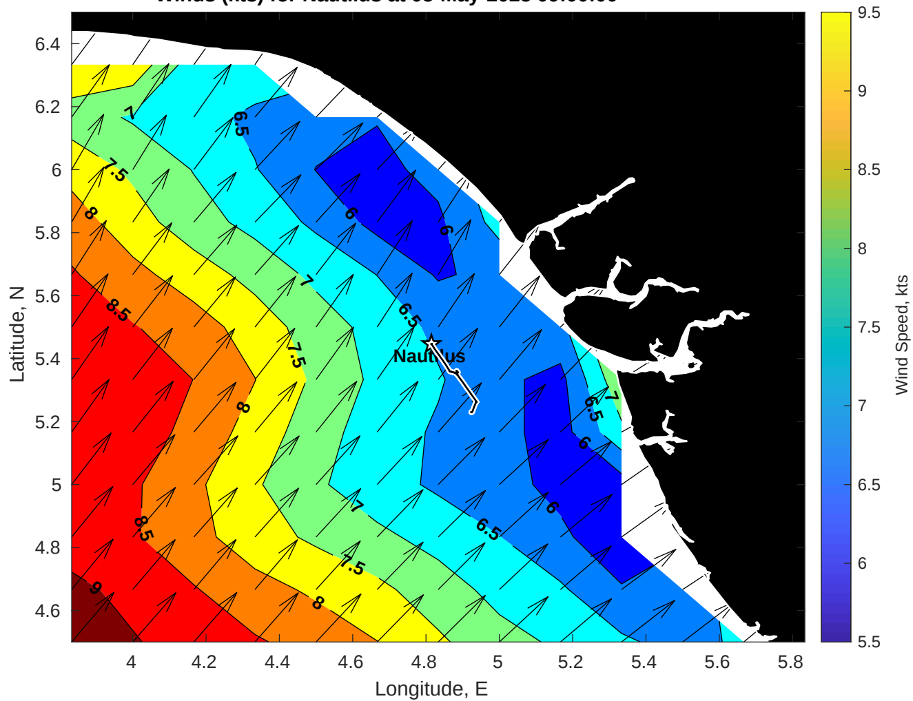
Winds (kts) for Nautilus at 05-May-2025 09:00:00
