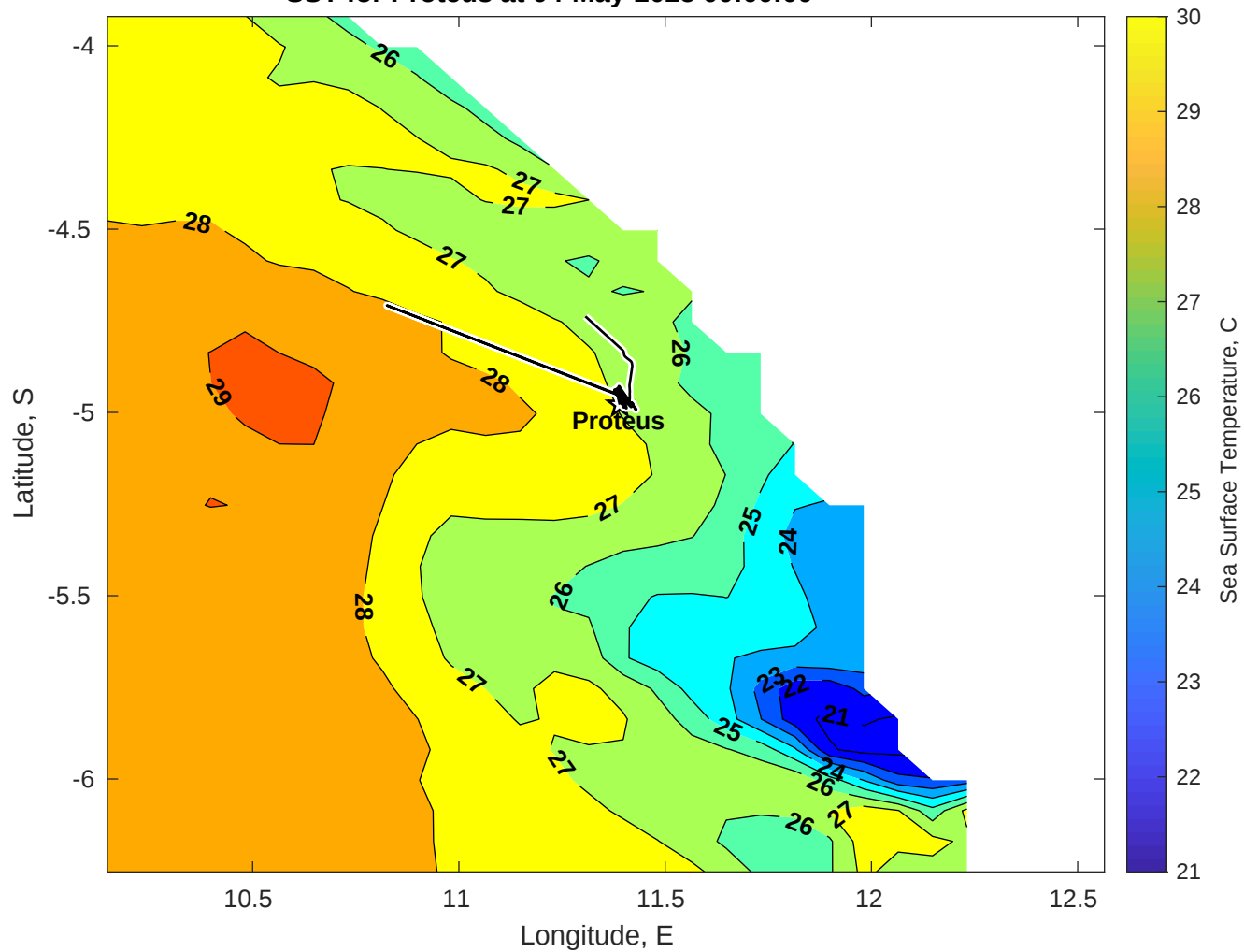
SST for Proteus at 04-May-2025 00:00:00
