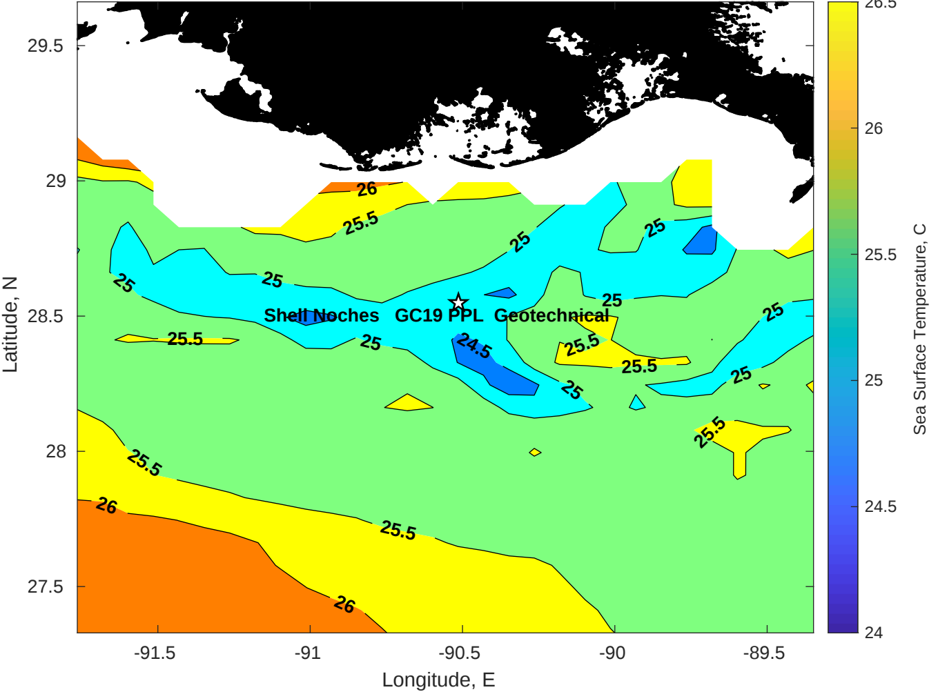
SST for Shell Noches GC19 PPL Geotechnical at 04-May-2025 00:00:00
