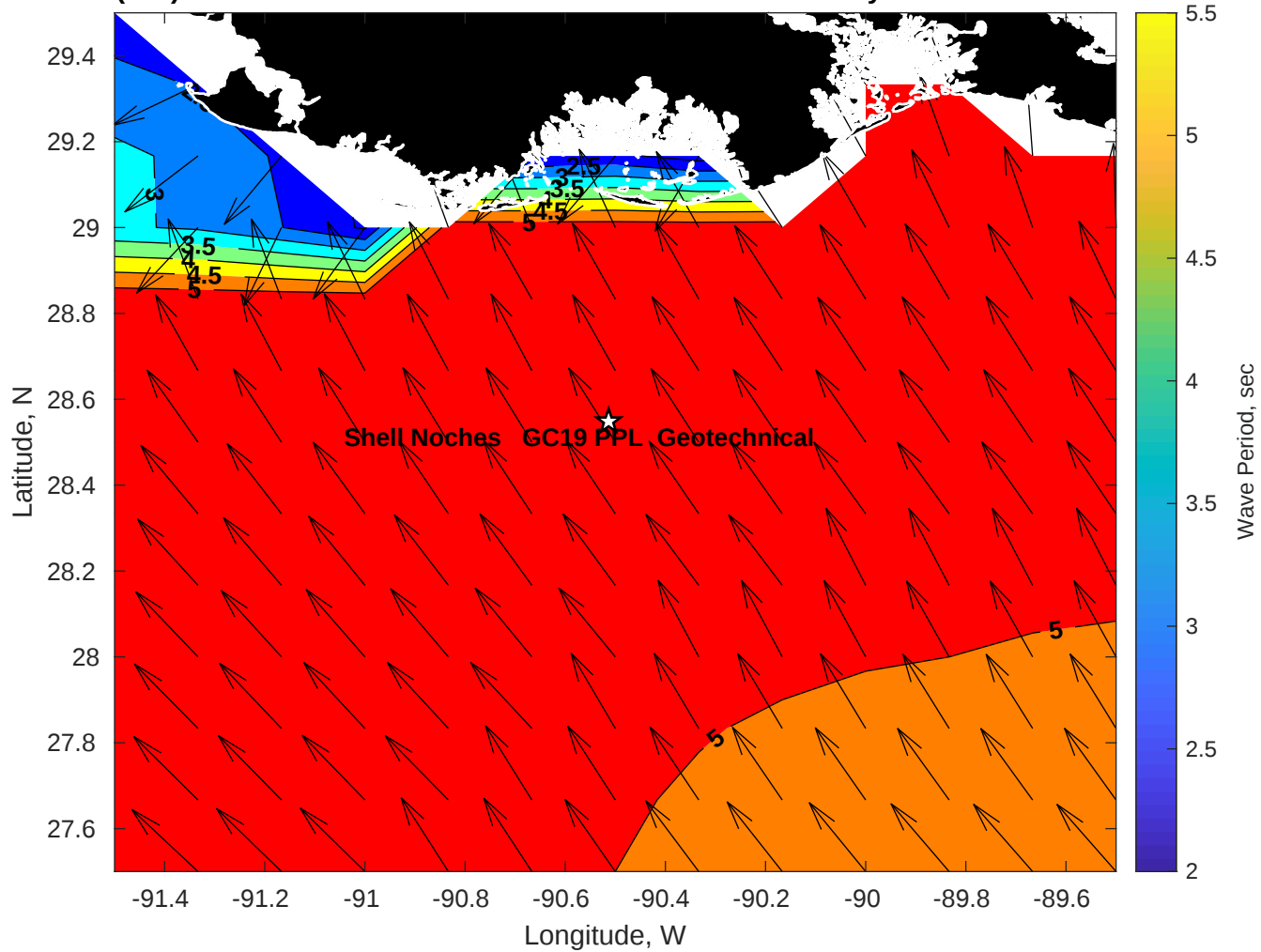
Wave Period (sec) for Shell Noches GC19 PPL Geotechnical at 05-May-2025 09:00:00
