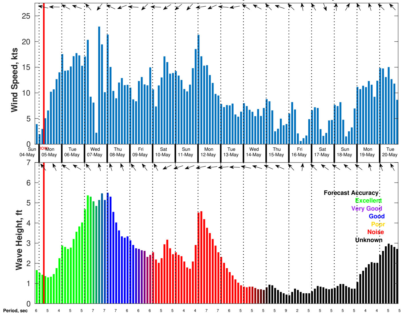
Wind & Wave Forecast for Shell Noches GC19 PPL Geotechnical from 04-May-2025 20:00:00 to 20-May-2025 20:00:00
