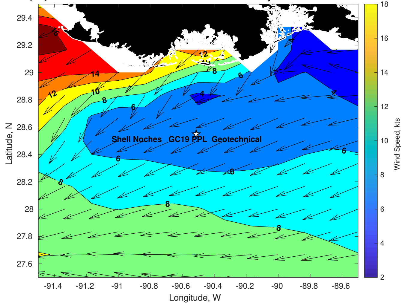
Winds (kts) for Shell Noches GC19 PPL Geotechnical at 05-May-2025 09:00:00
