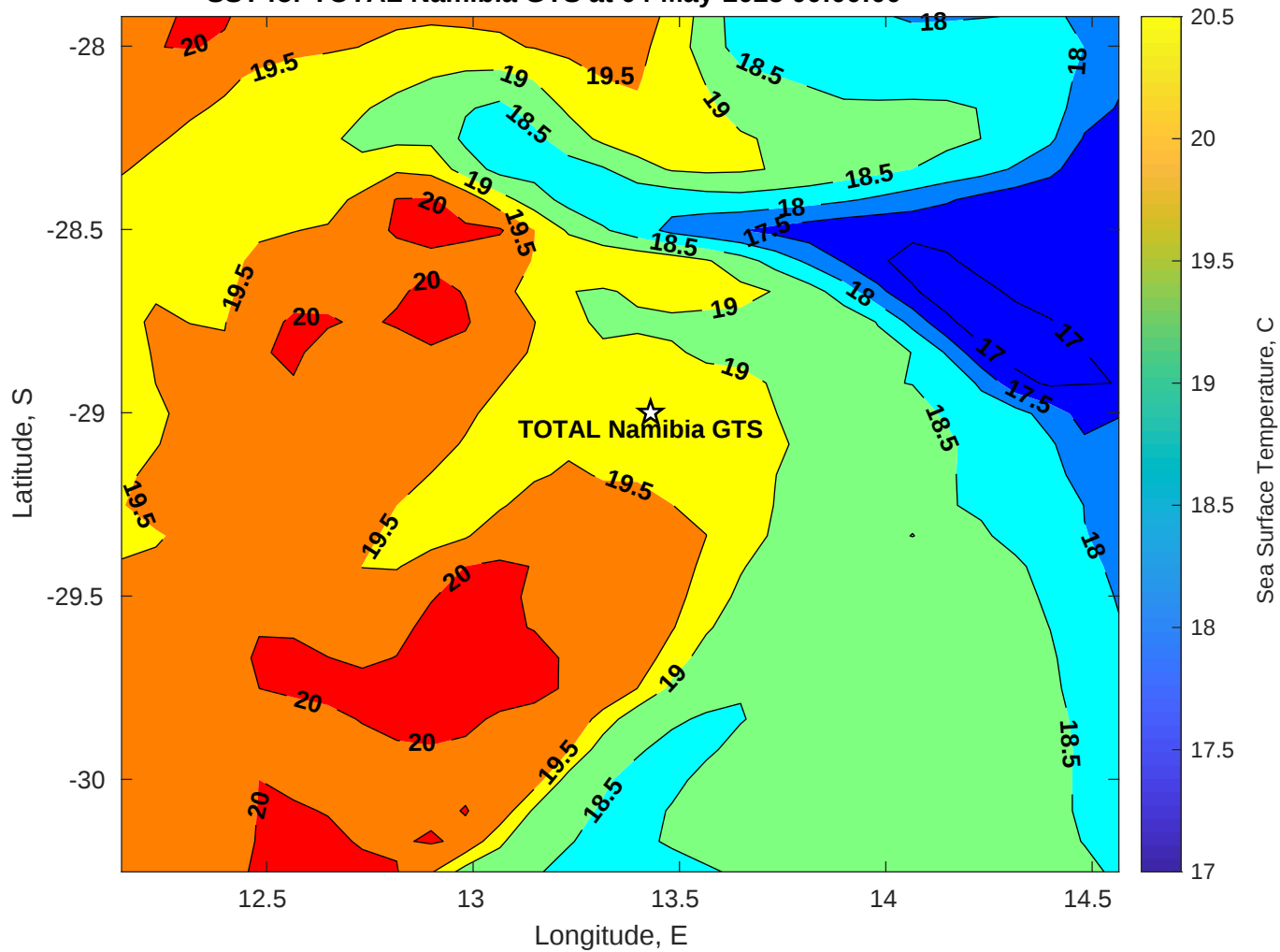
SST for TOTAL Namibia GTS at 04-May-2025 00:00:00
