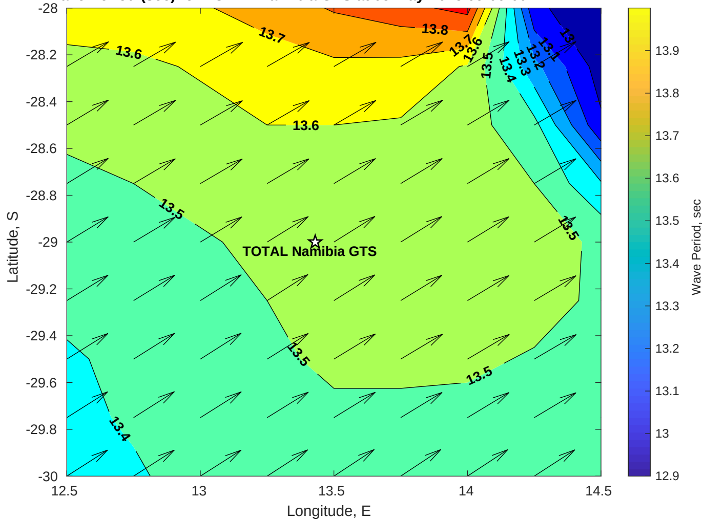
Wave Period (sec) for TOTAL Namibia GTS at 05-May-2025 09:00:00
