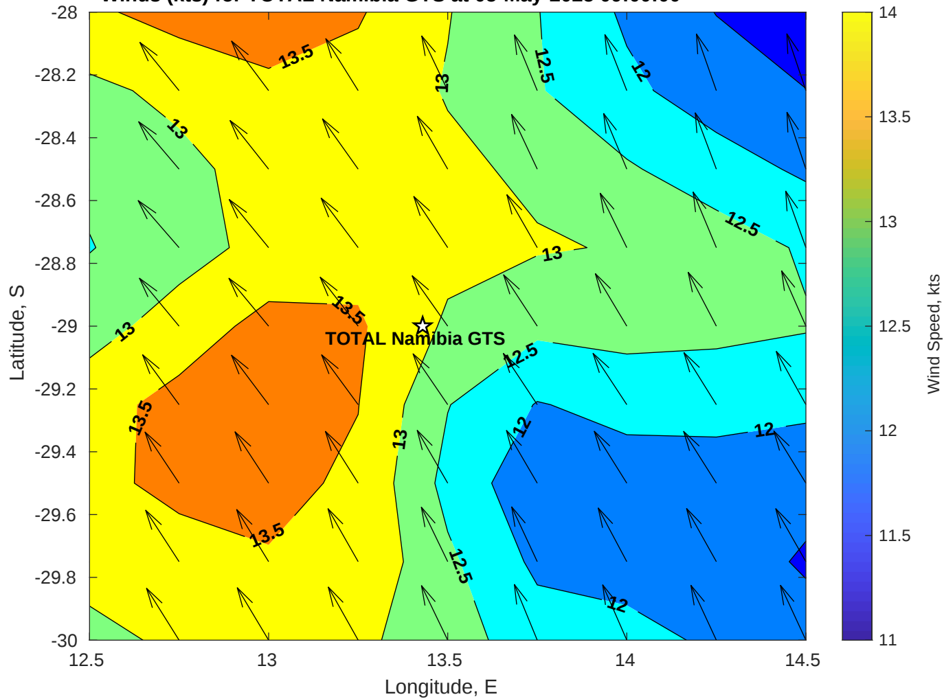
Winds (kts) for TOTAL Namibia GTS at 05-May-2025 09:00:00
