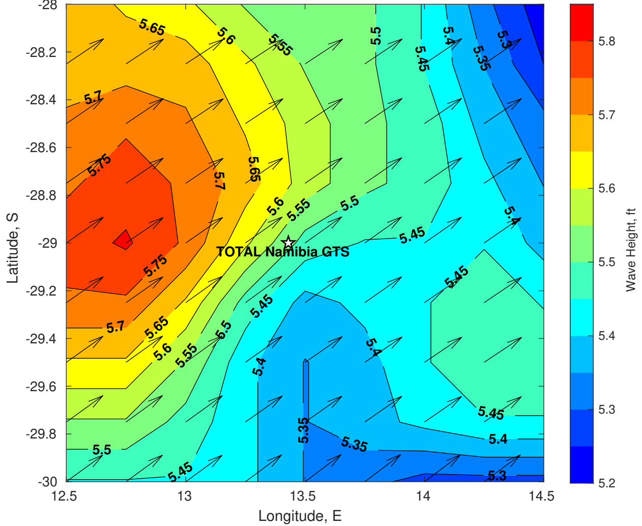
Wave Height (ft) for TOTAL Namibia GTS at 05-May-2025 09:00:00
