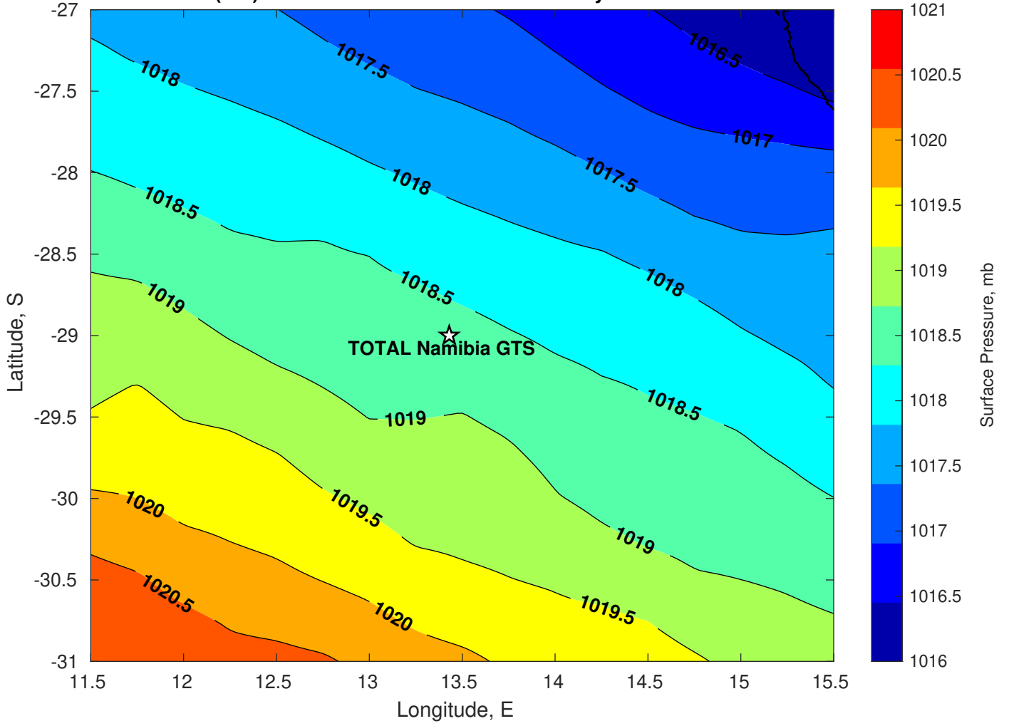
Surface Pressure (mb) for TOTAL Namibia GTS at 07-May-2025 00:00:00
