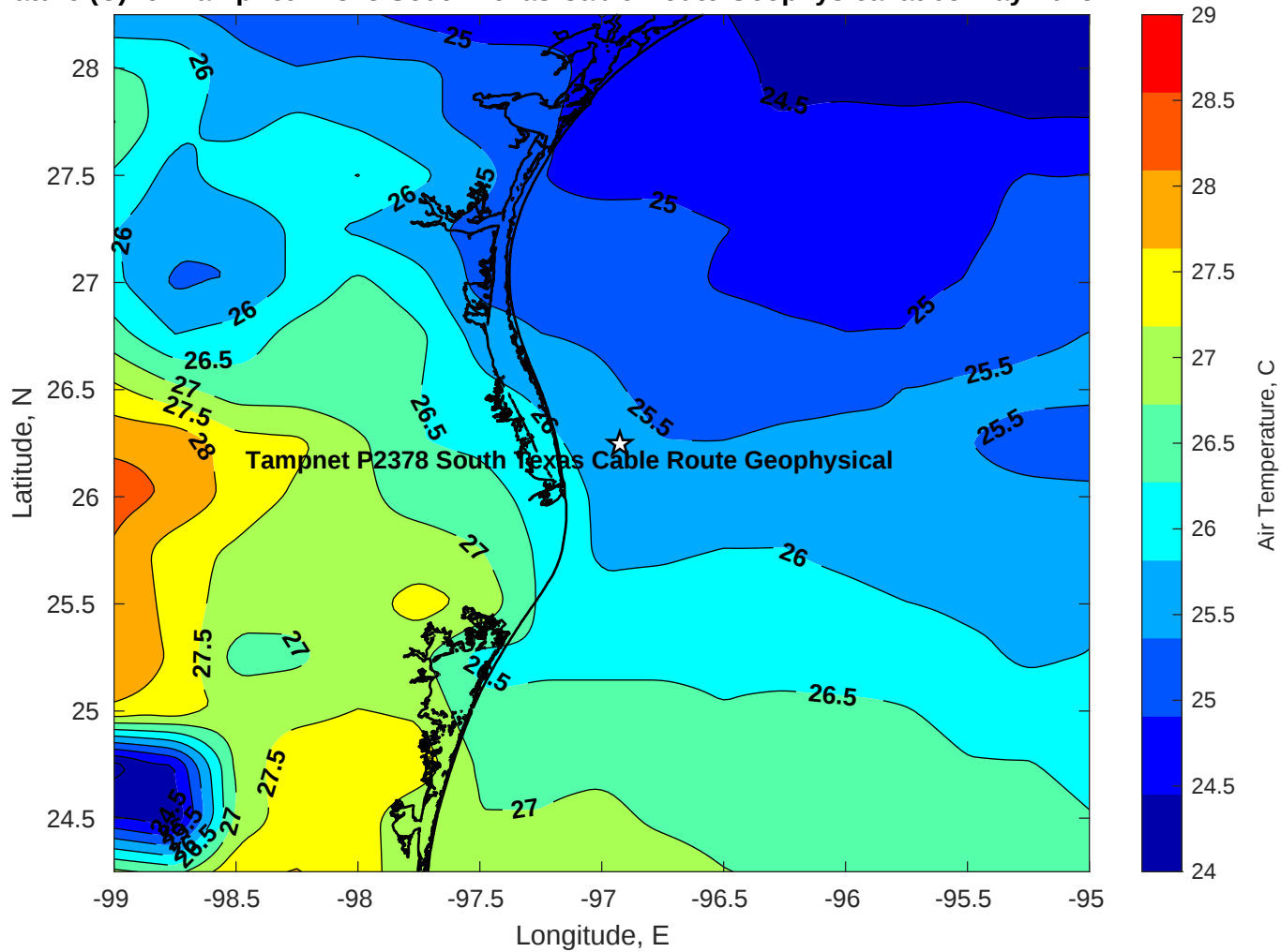
Air Temperature (C) for Tampnet P2378 South Texas Cable Route Geophysical at 05-May-2025
