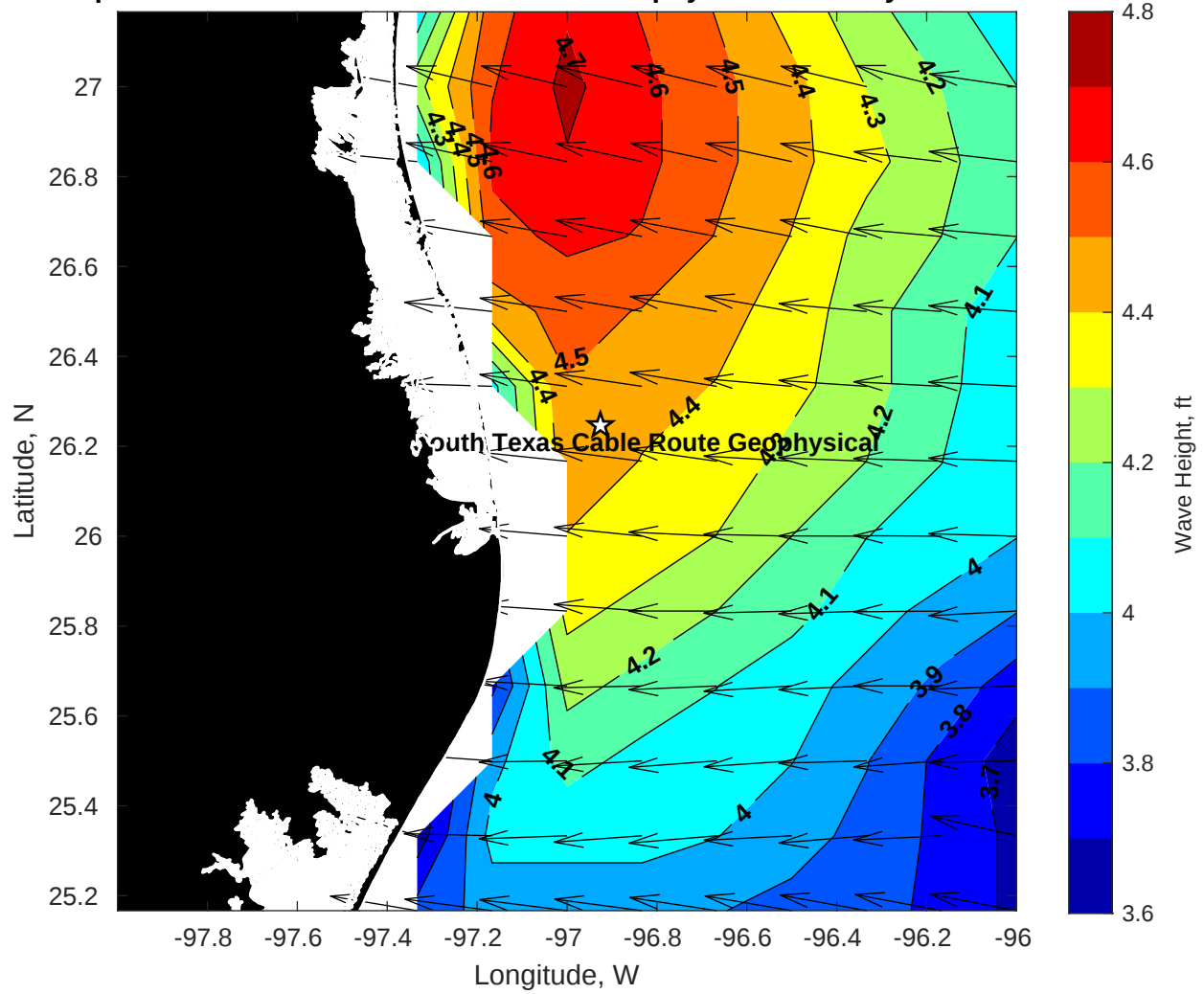
Wave Height (ft) for Tampnet P2378 South Texas Cable Route Geophysical at 05-May-2025 09:00:00
