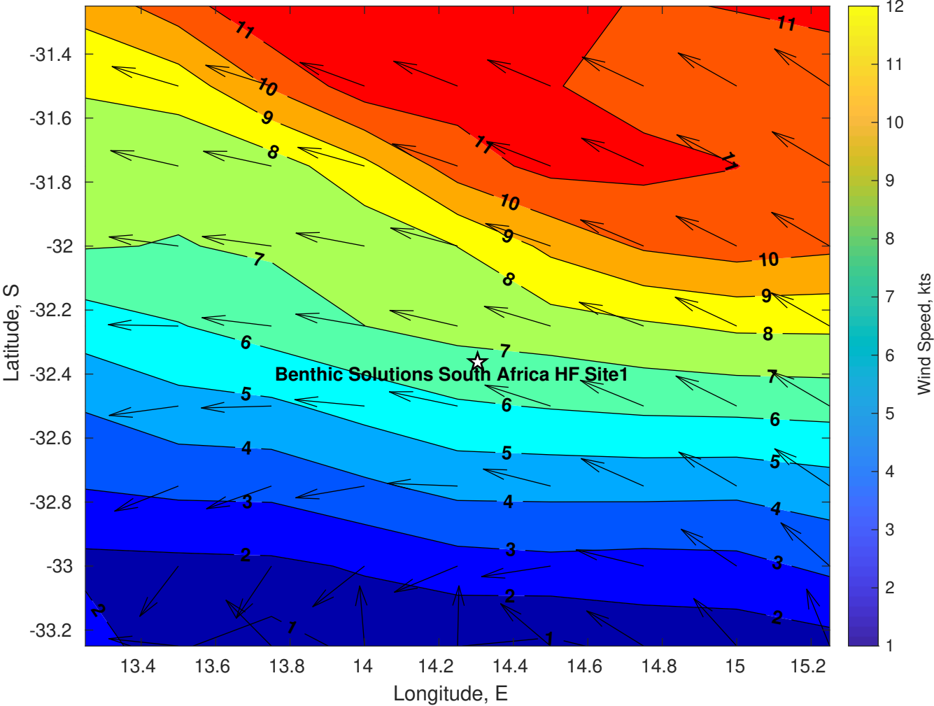
Winds (kts) for Benthic Solutions South Africa HF Site1 at 06-May-2025 09:00:00
