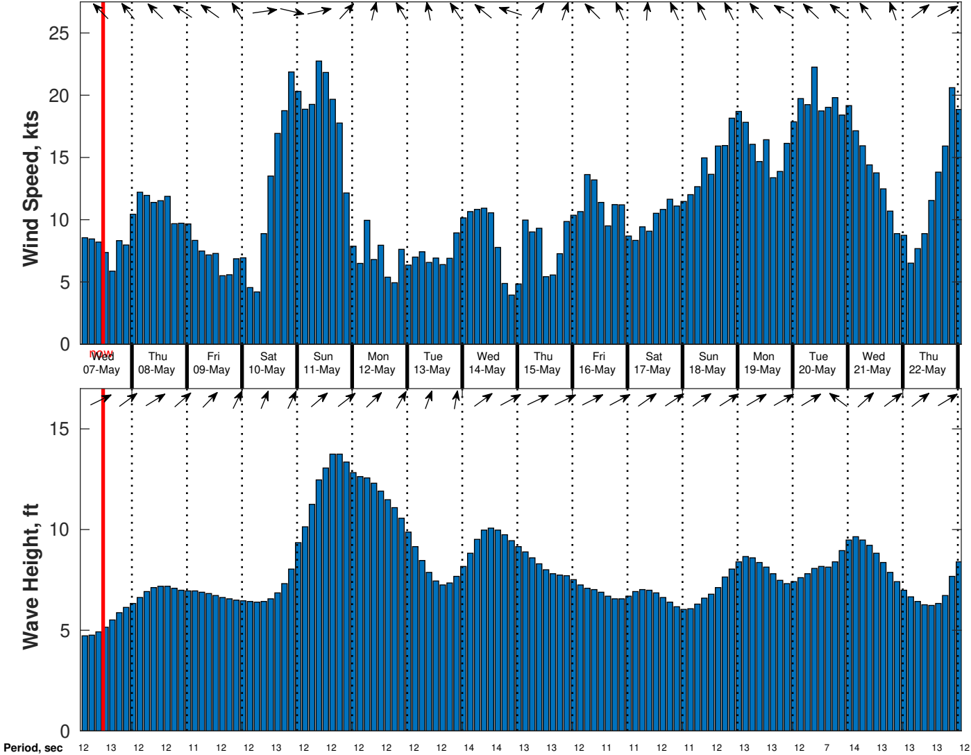
Wind & Wave Forecast for Benthic Solutions South Africa HF Site1 from 06-May-2025 02:00:00 to 22-May-2025 02:00:00
