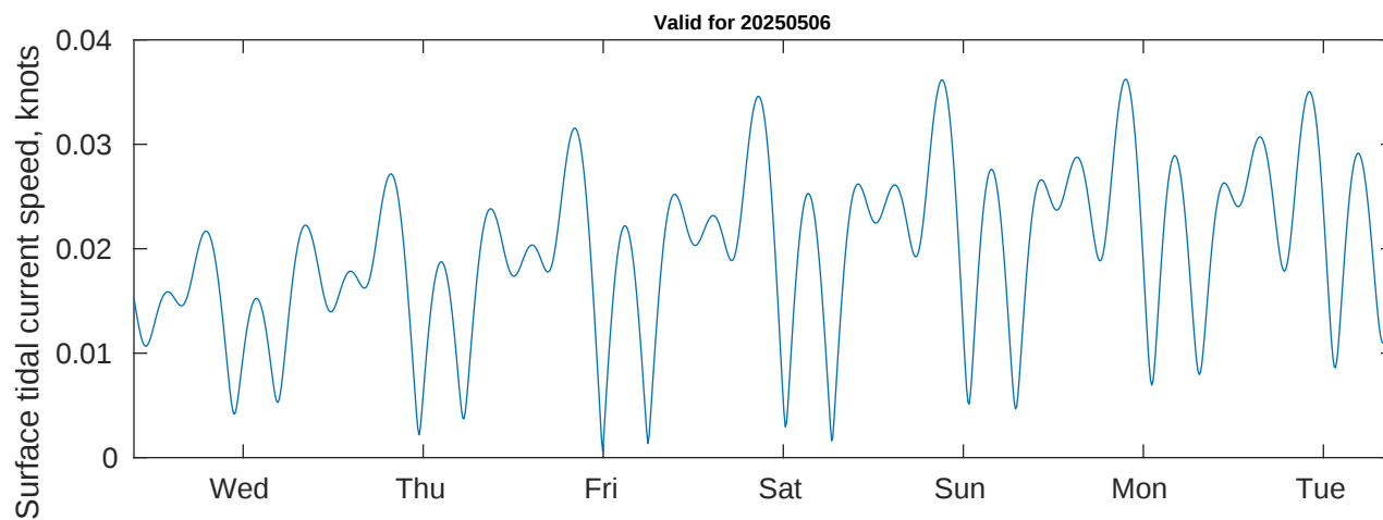
Tidal Currents and Heights for Benthic Solutions South Africa HF Site1 at 20250506
