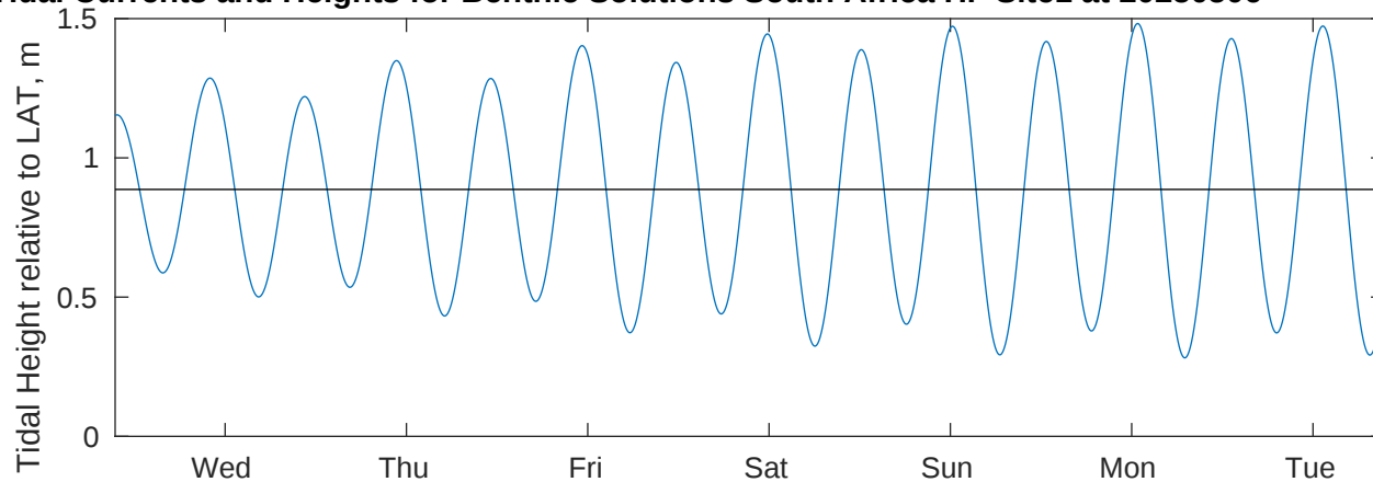
Tidal Currents and Heights for Benthic Solutions South Africa HF Site1 at 20250506
