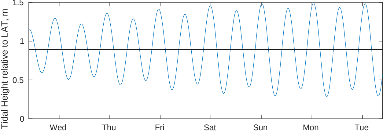
Tidal Currents and Heights for Benthic Solutions South Africa HF Site2 at 20250506
