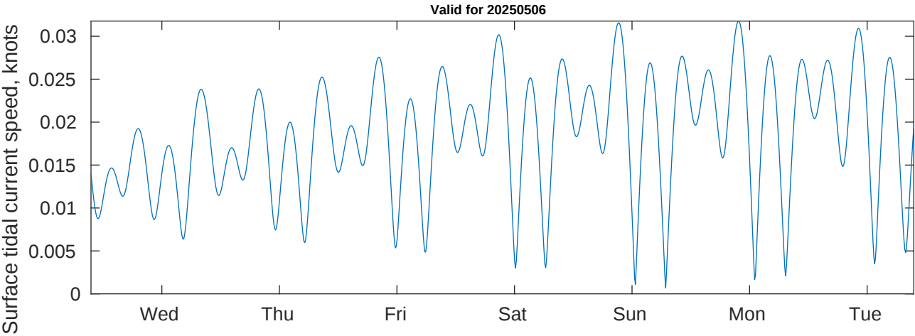
Tidal Currents and Heights for Benthic Solutions South Africa HF Site2 at 20250506
