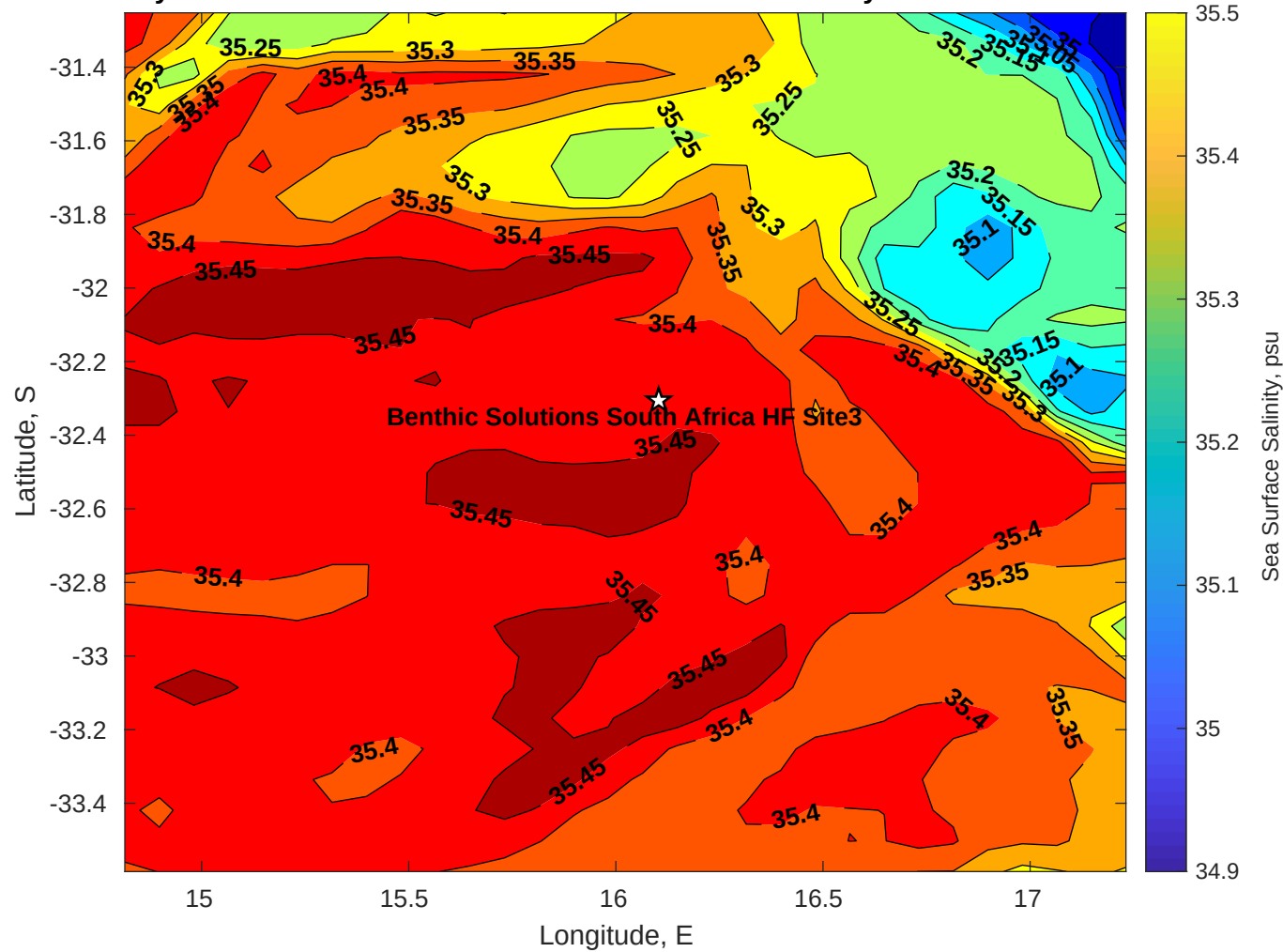
Surface Salinity for Benthic Solutions South Africa HF Site3 at 05-May-2025 00:00:00
