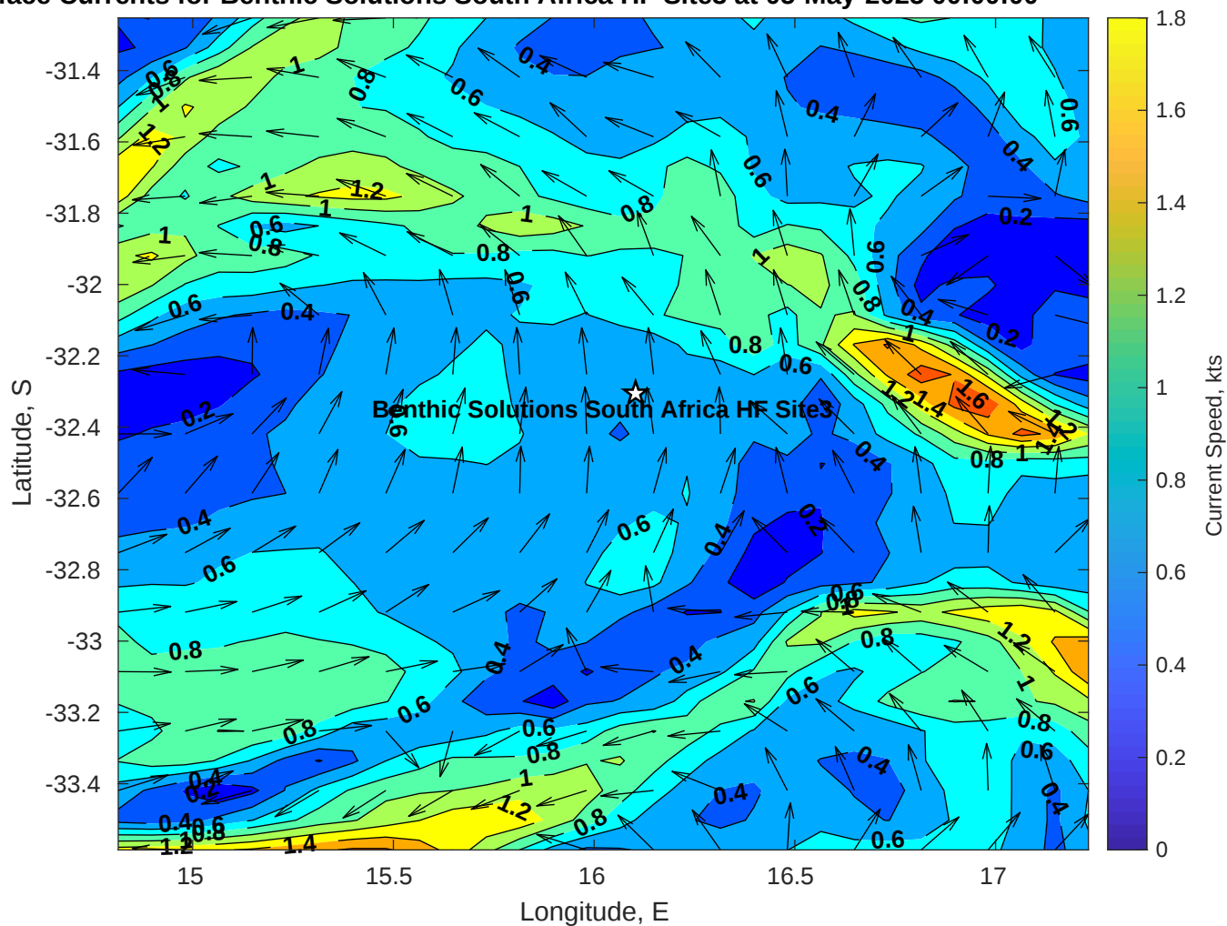
Surface Currents for Benthic Solutions South Africa HF Site3 at 05-May-2025 00:00:00
