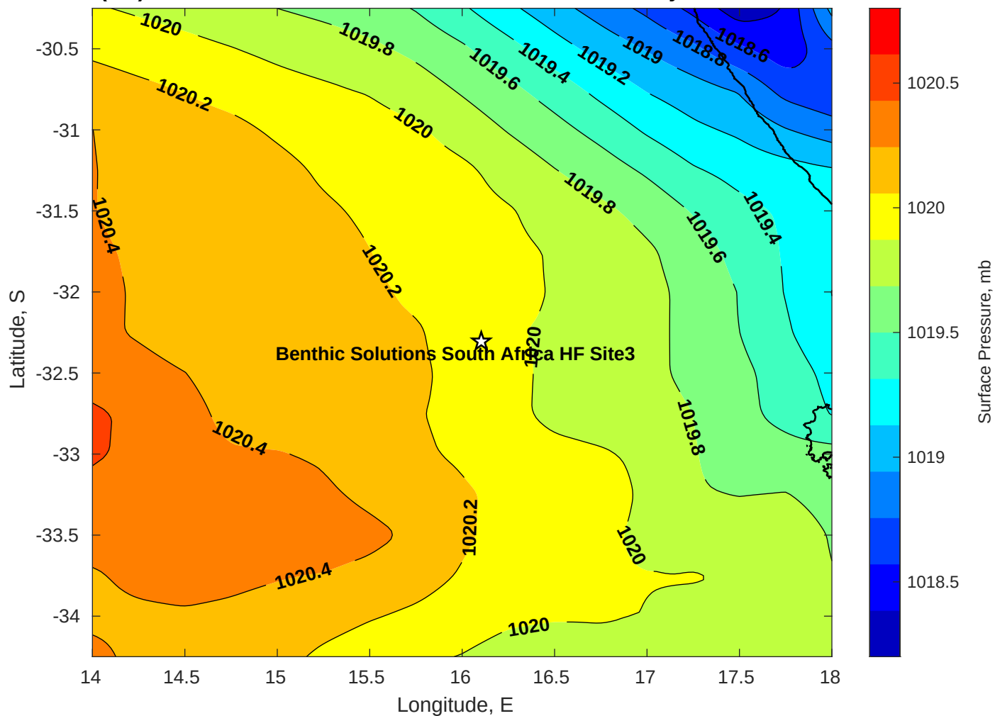
Surface Pressure (mb) for Benthic Solutions South Africa HF Site3 at 06-May-2025 00:00:00
