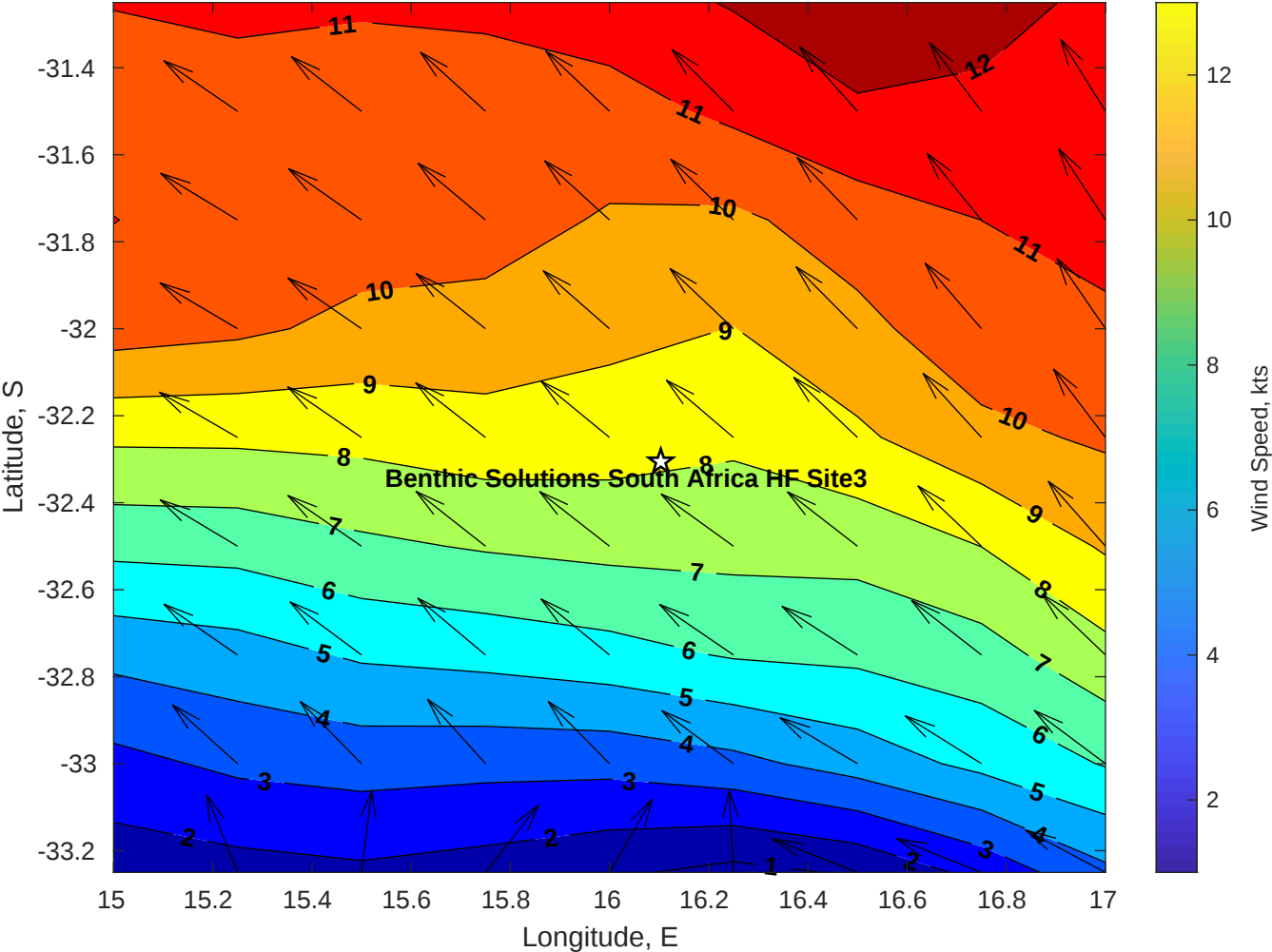
Winds (kts) for Benthic Solutions South Africa HF Site3 at 06-May-2025 09:00:00
