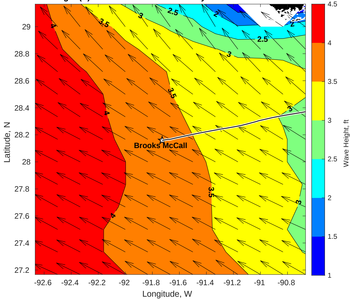
Wave Height (ft) for Brooks McCall at 06-May-2025 09:00:00
