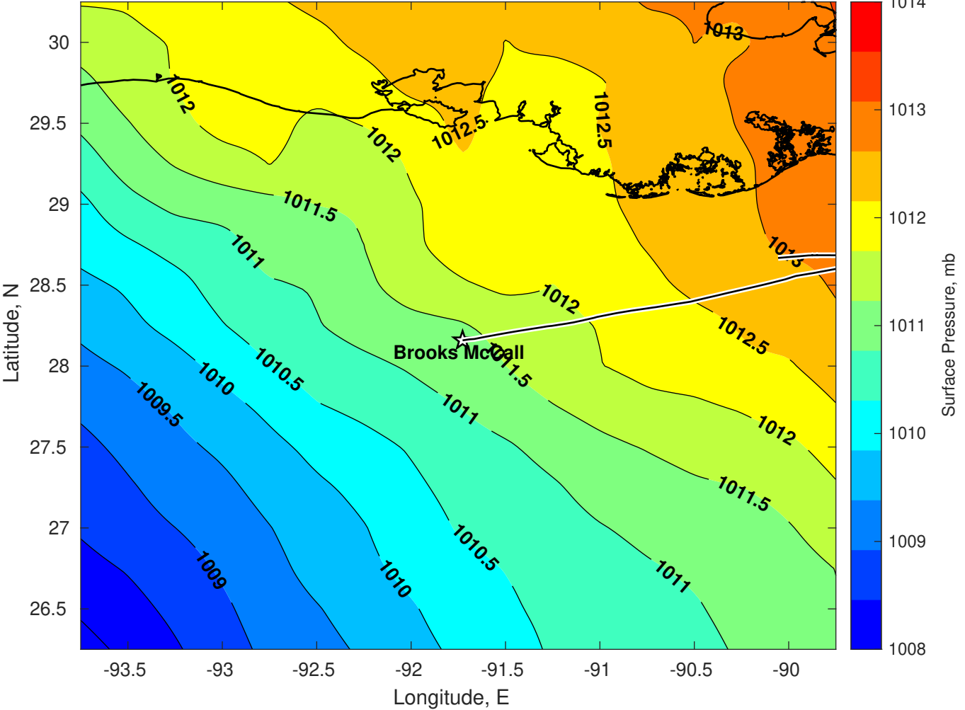
Surface Pressure (mb) for Brooks McCall at 06-May-2025 00:00:00
