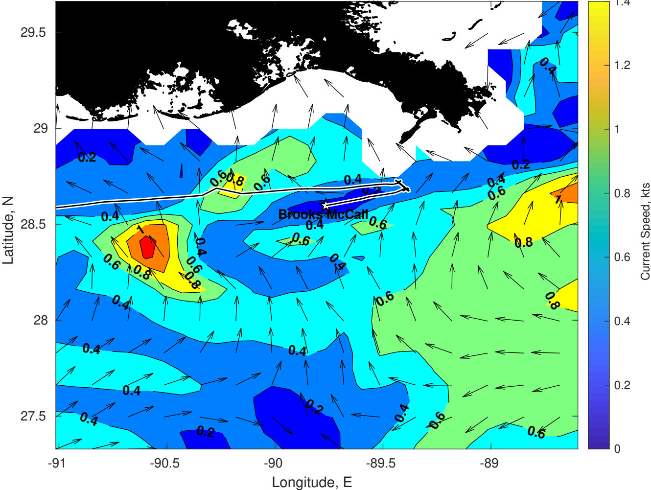
Surface Currents for Brooks McCall at 05-May-2025 00:00:00
