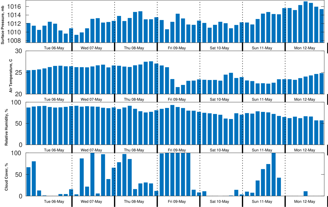
Met Forecast for Brooks McCall from 06-May-2025 00:00:00 to 13-May-2025 00:00:00
