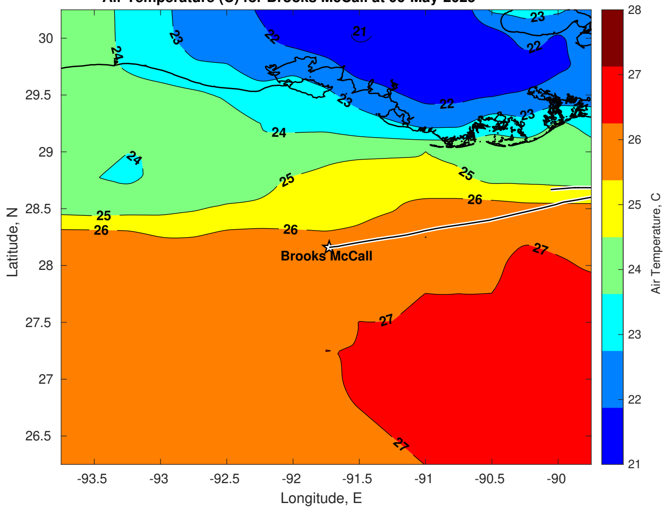
Air Temperature (C) for Brooks McCall at 06-May-2025
