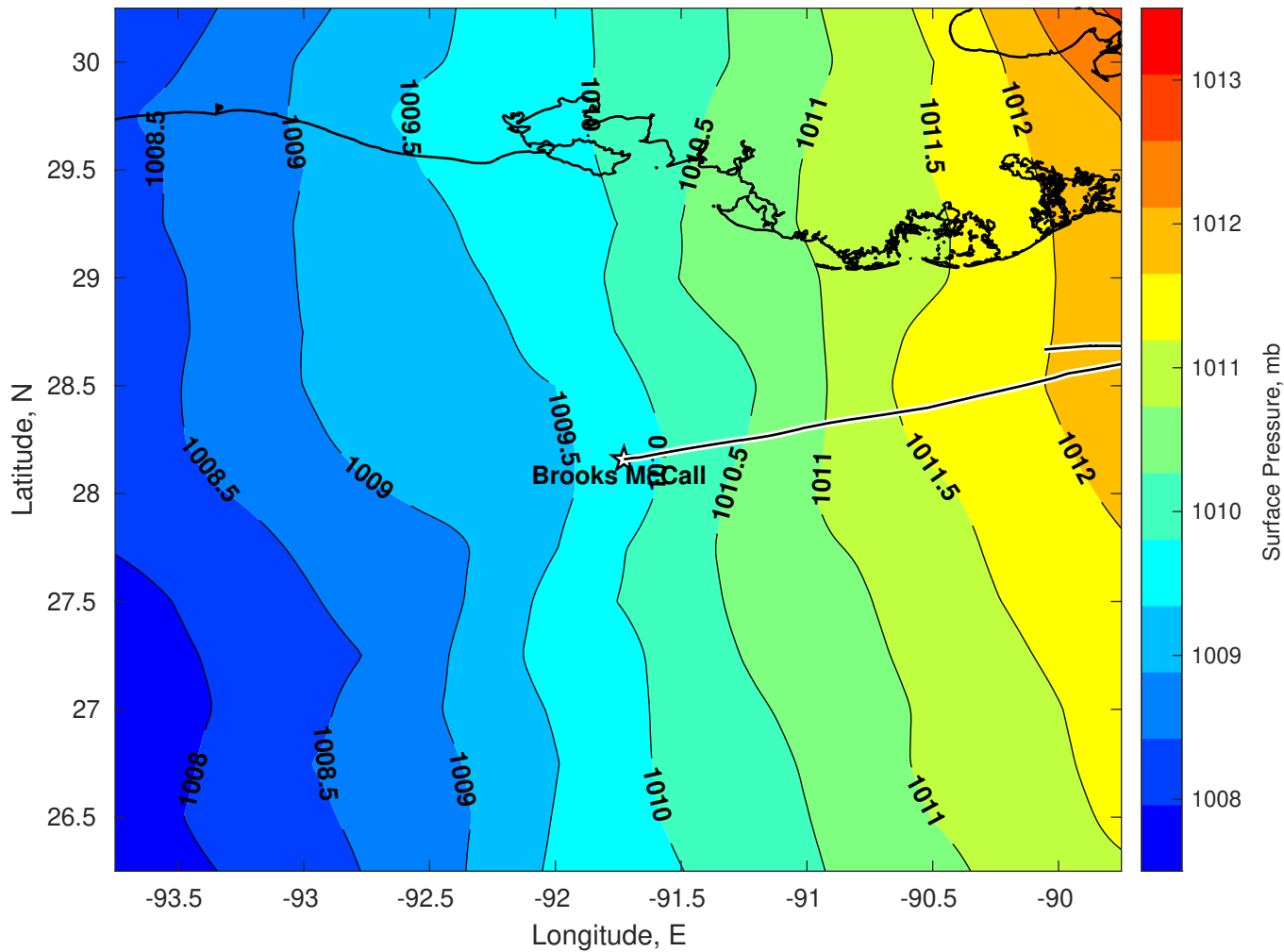
Surface Pressure (mb) for Brooks McCall at 07-May-2025 00:00:00
