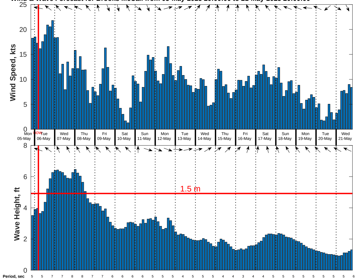
Wind & Wave Forecast for Brooks McCall from 05-May-2025 20:00:00 to 21-May-2025 20:00:00
