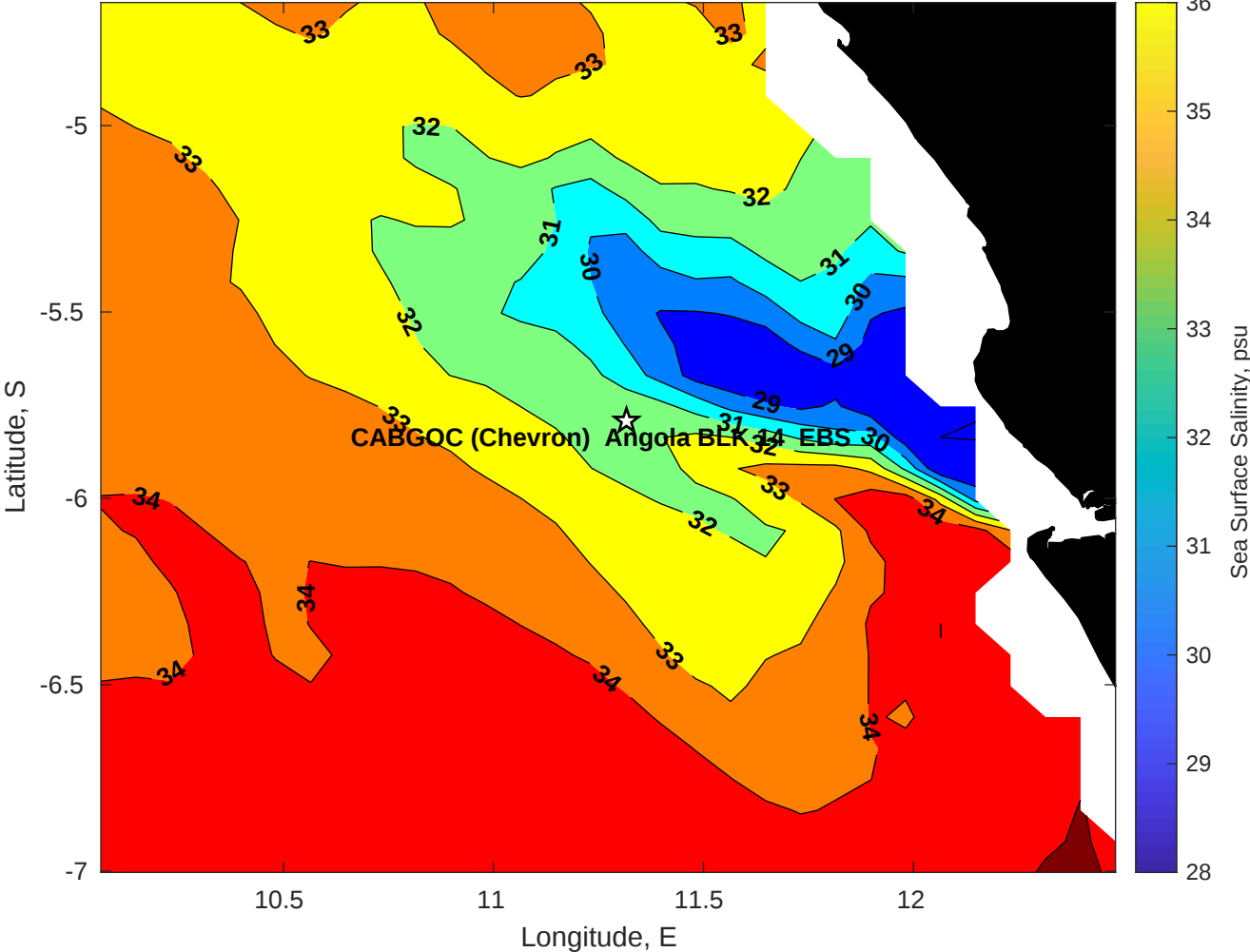
Surface Salinity for CABGOC (Chevron) Angola BLK 14 EBS at 05-May-2025 00:00:00
