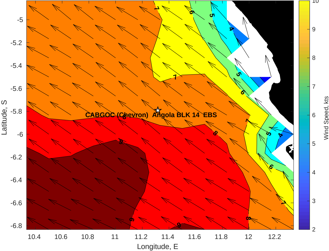
Winds (kts) for CABGOC (Chevron) Angola BLK 14 EBS at 06-May-2025 09:00:00
