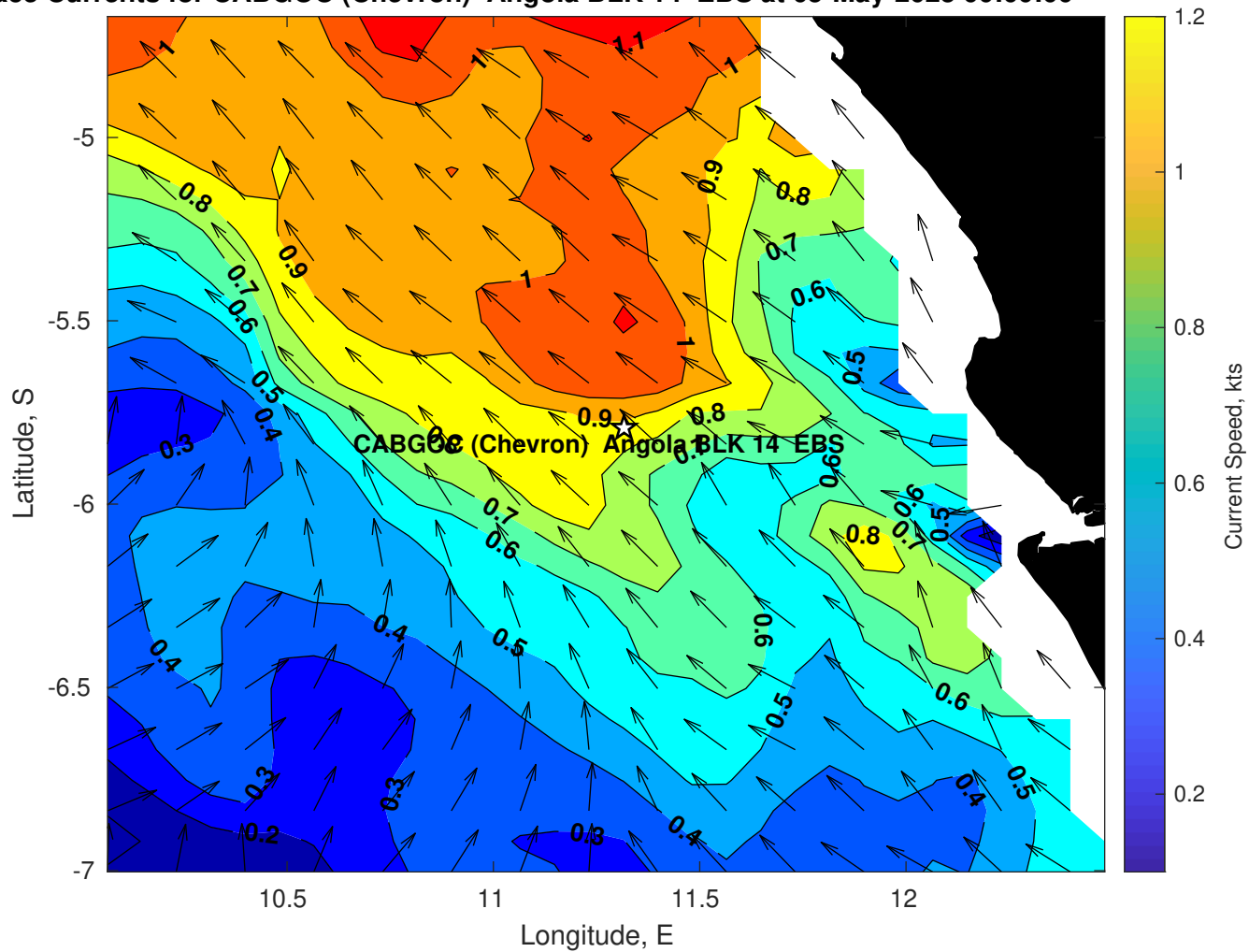
Surface Currents for CABGOC (Chevron) Angola BLK 14 EBS at 05-May-2025 00:00:00
