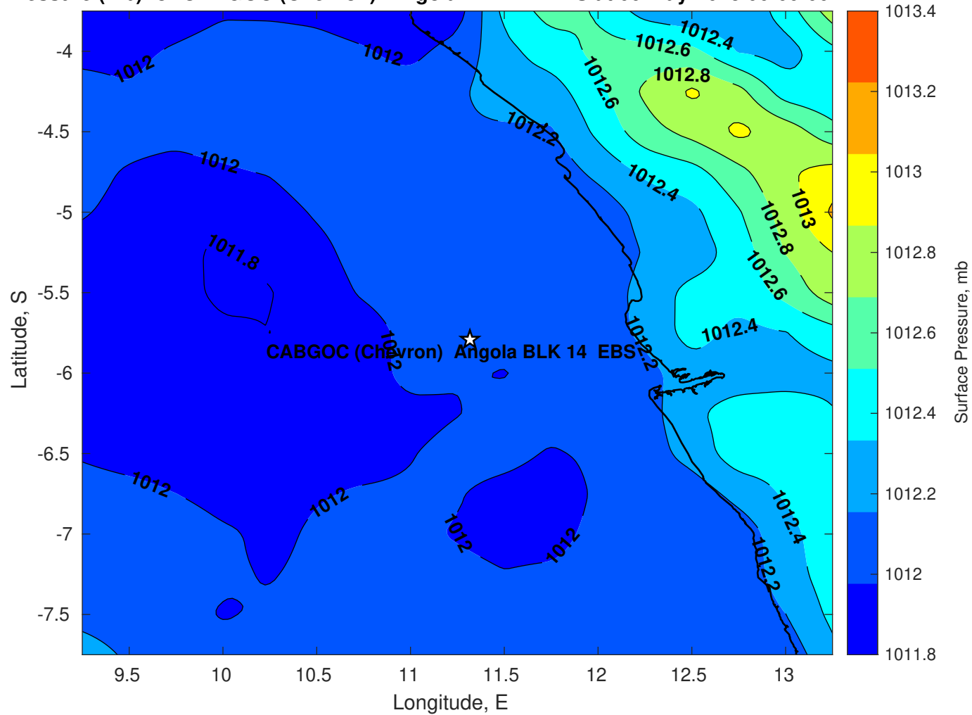
Surface Pressure (mb) for CABGOC (Chevron) Angola BLK 14 EBS at 06-May-2025 00:00:00
