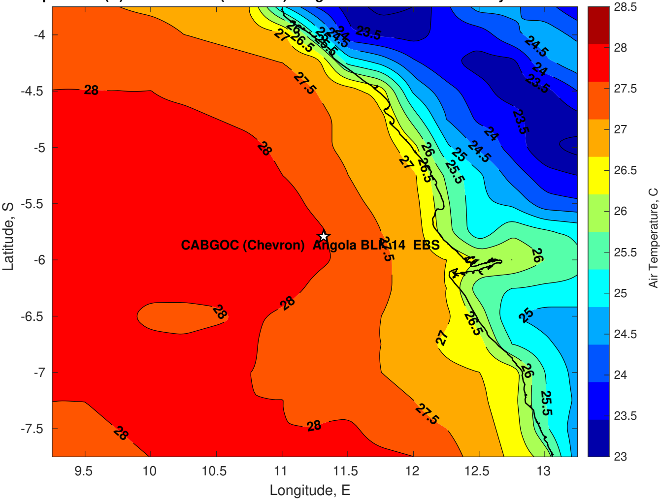
Air Temperature (C) for CABGOC (Chevron) Angola BLK 14 EBS at 06-May-2025
