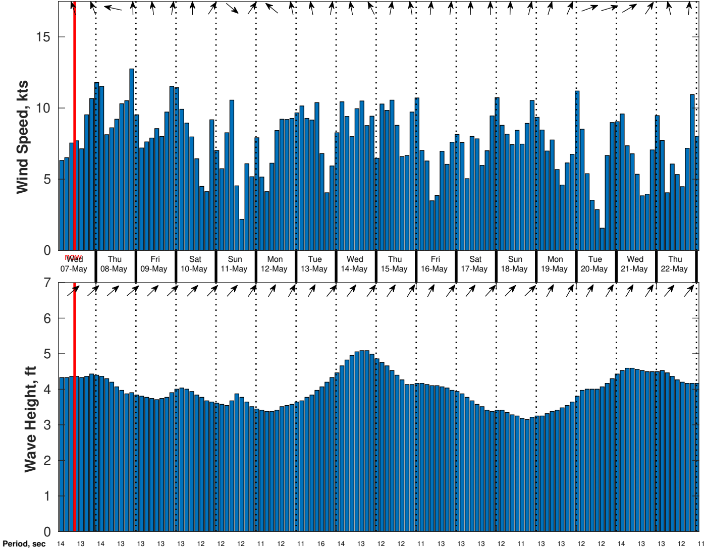
Wind & Wave Forecast for CABGOC (Chevron) Angola BLK 14 EBS from 06-May-2025 02:00:00 to 22-May-2025 02:00:00
