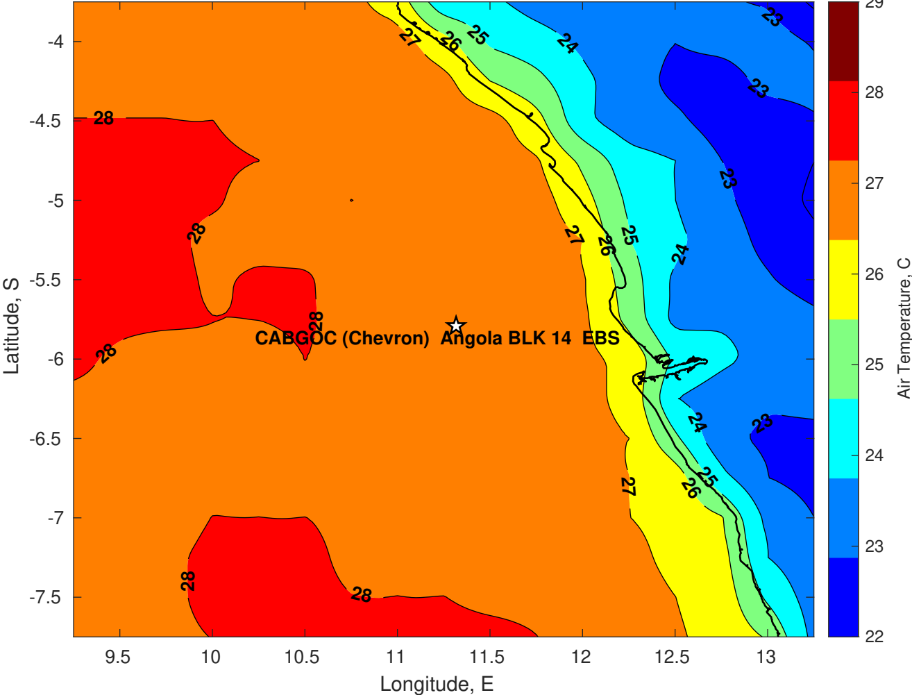
Air Temperature (C) for CABGOC (Chevron) Angola BLK 14 EBS at 06-May-2025
