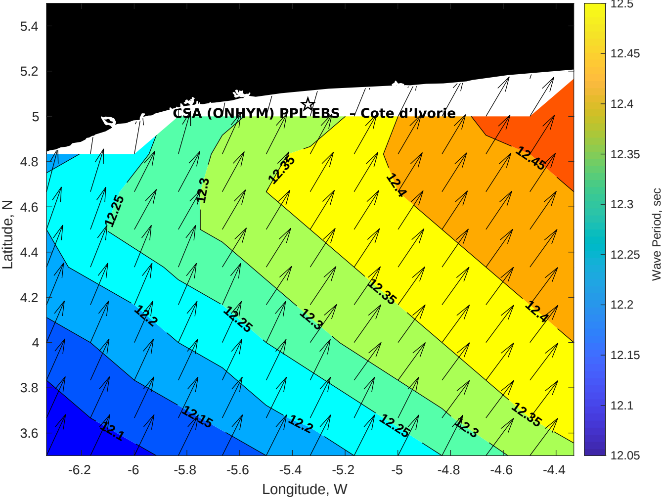
Wave Period (sec) for CSA (ONHYM) PPL EBS - Cote d'Ivoire at 06-May-2025 09:00:00
