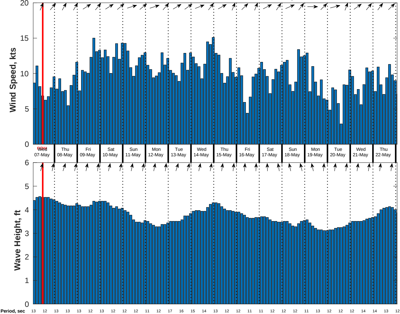
Wind & Wave Forecast for CSA (ONHYM) PPL EBS - Cote d'Ivoire from 06-May-2025 01:00:00 to 22-May-2025 01:00:00
