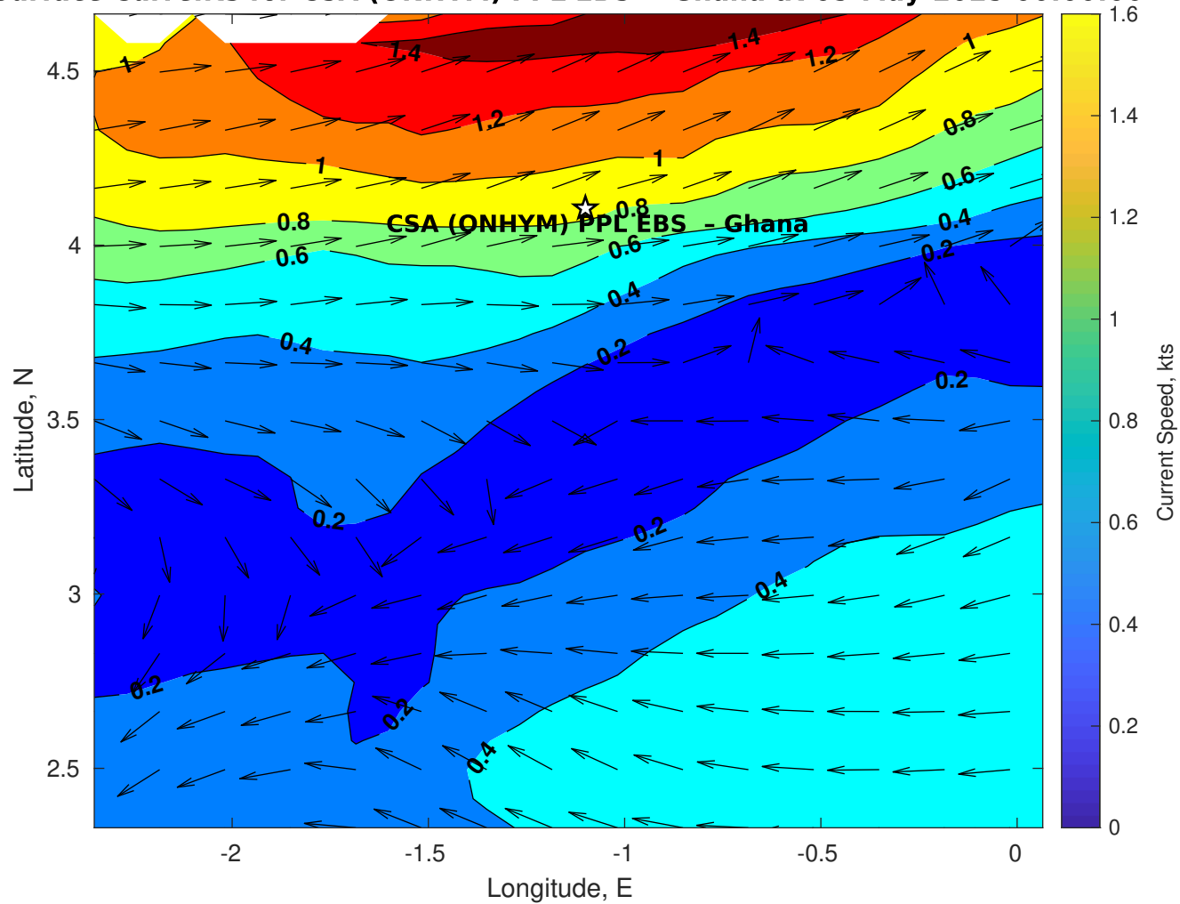
Surface Currents for CSA (ONHYM) PPL EBS - Ghana at 05-May-2025 00:00:00
