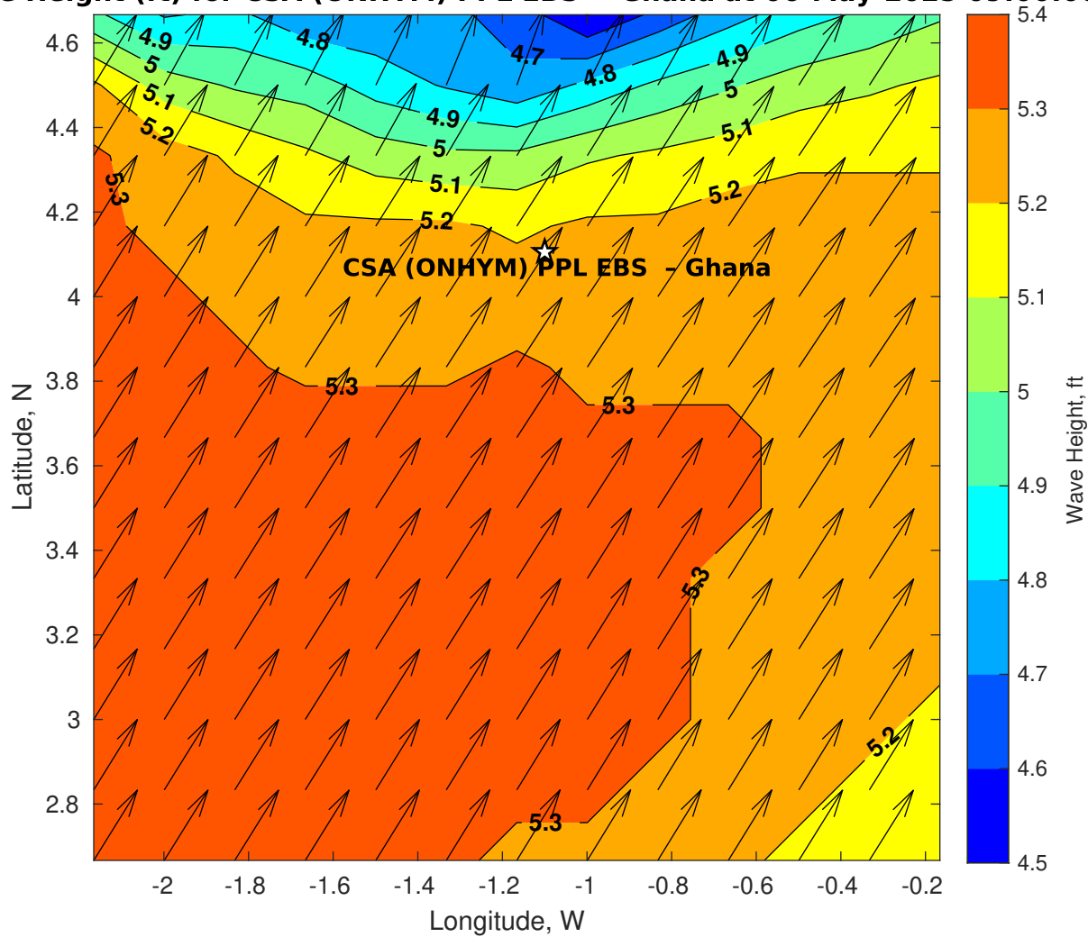
Wave Height (ft) for CSA (ONHYM) PPL EBS - Ghana at 06-May-2025 09:00:00
