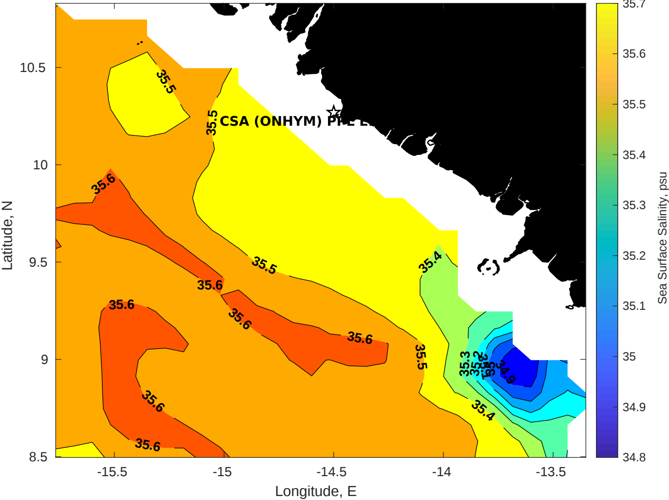
Surface Salinity for CSA (ONHYM) PPL EBS - Guinea at 05-May-2025 00:00:00
