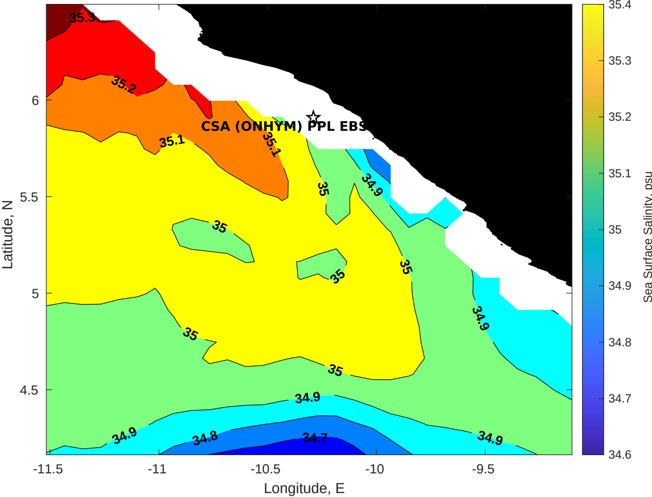
Surface Salinity for CSA (ONHYM) PPL EBS - Liberia at 05-May-2025 00:00:00
