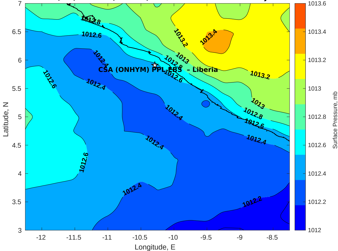
Surface Pressure (mb) for CSA (ONHYM) PPL EBS - Liberia at 07-May-2025 00:00:00
