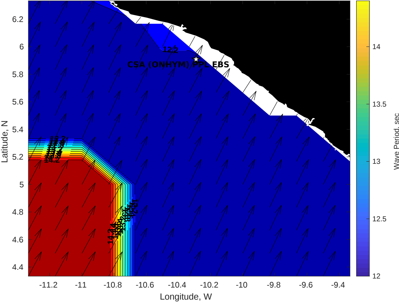
Wave Period (sec) for CSA (ONHYM) PPL EBS - Liberia at 06-May-2025 09:00:00
