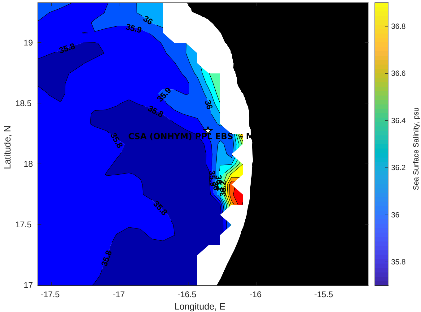
Surface Salinity for CSA (ONHYM) PPL EBS - Mauritania at 05-May-2025 00:00:00
