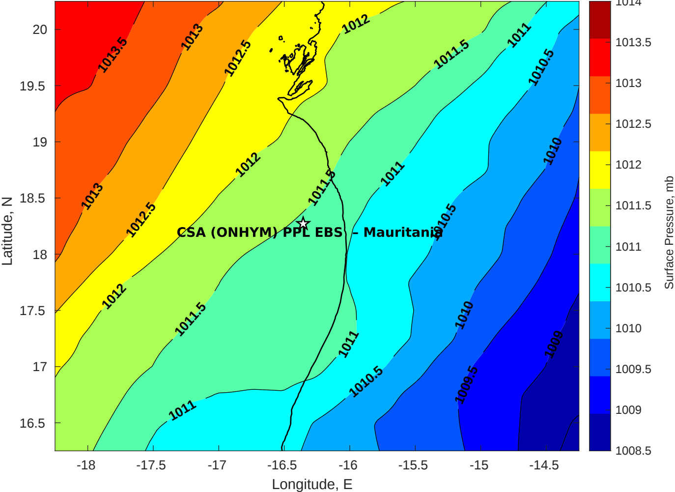
Surface Pressure (mb) for CSA (ONHYM) PPL EBS - Mauritania at 06-May-2025 00:00:00
