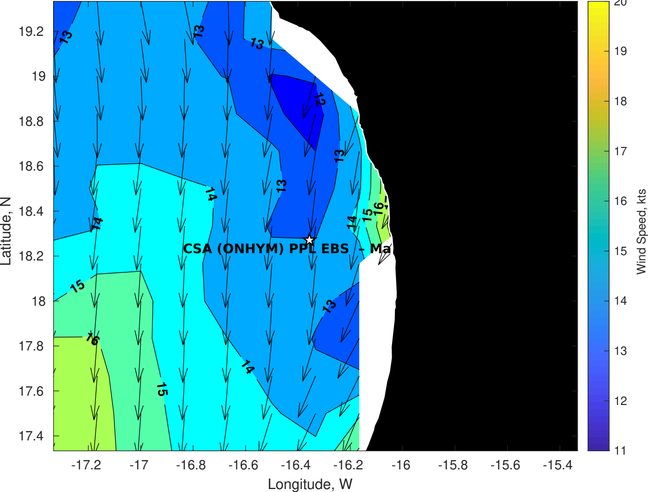
Winds (kts) for CSA (ONHYM) PPL EBS - Mauritania at 06-May-2025 09:00:00
