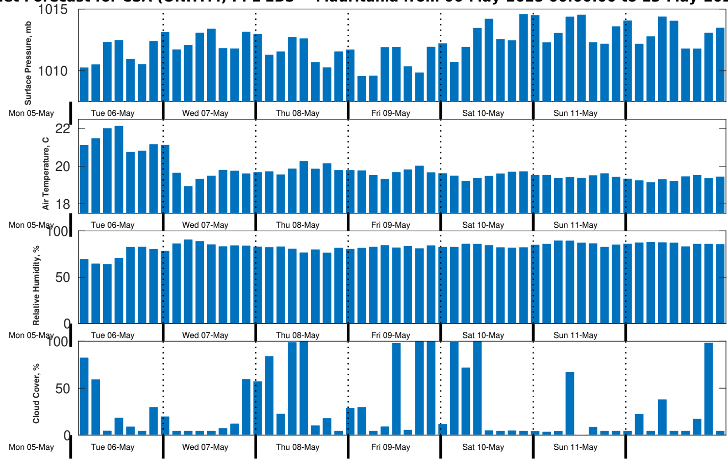
Met Forecast for CSA (ONHYM) PPL EBS - Mauritania from 06-May-2025 00:00:00 to 13-May-2025 00:00:00
