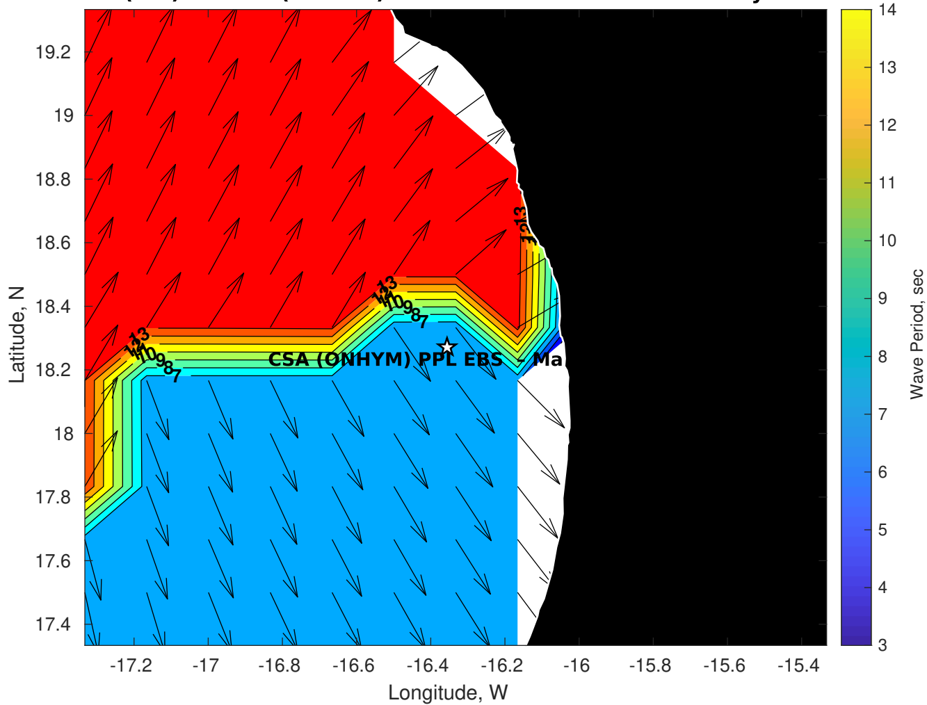
Wave Period (sec) for CSA (ONHYM) PPL EBS - Mauritania at 06-May-2025 09:00:00
