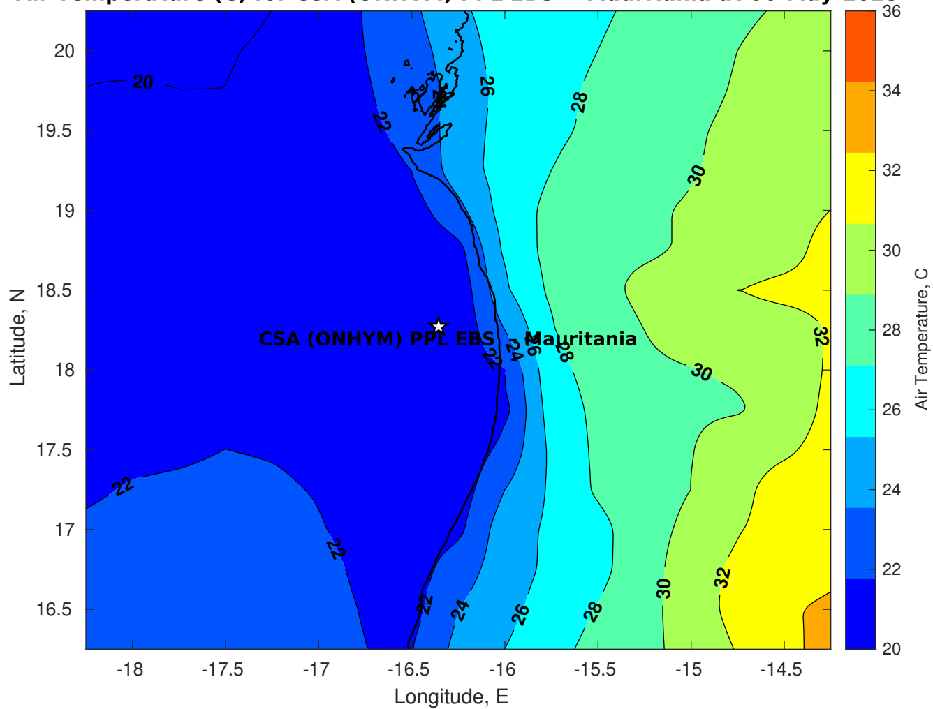
Air Temperature (C) for CSA (ONHYM) PPL EBS - Mauritania at 06-May-2025
