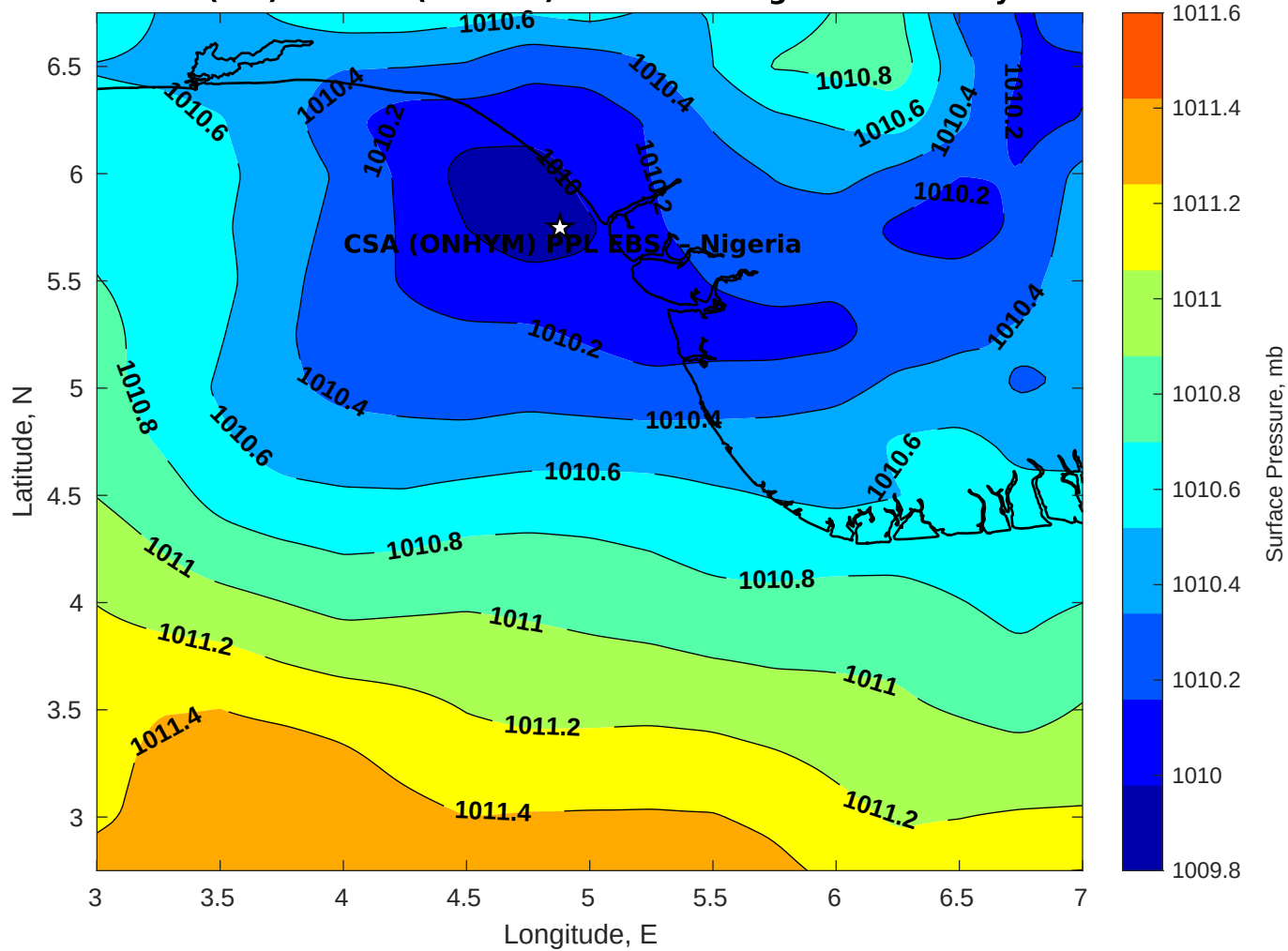
Surface Pressure (mb) for CSA (ONHYM) PPL EBS - Nigeria at 07-May-2025 00:00:00
