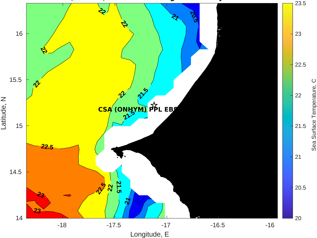
SST for CSA (ONHYM) PPL EBS - Senegal at 05-May-2025 00:00:00
