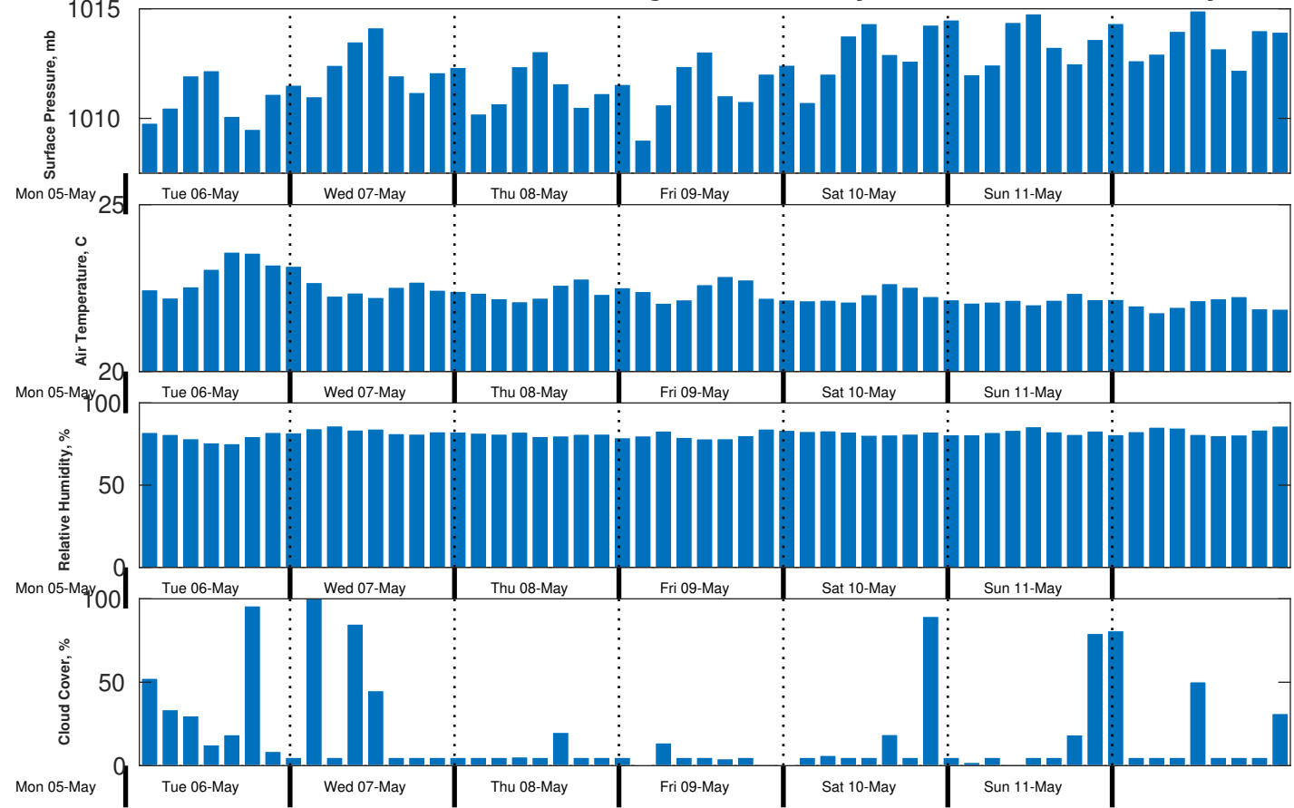
Met Forecast for CSA (ONHYM) PPL EBS - Senegal from 06-May-2025 00:00:00 to 13-May-2025 00:00:00
