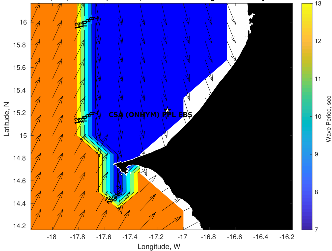
Wave Period (sec) for CSA (ONHYM) PPL EBS - Senegal at 06-May-2025 09:00:00
