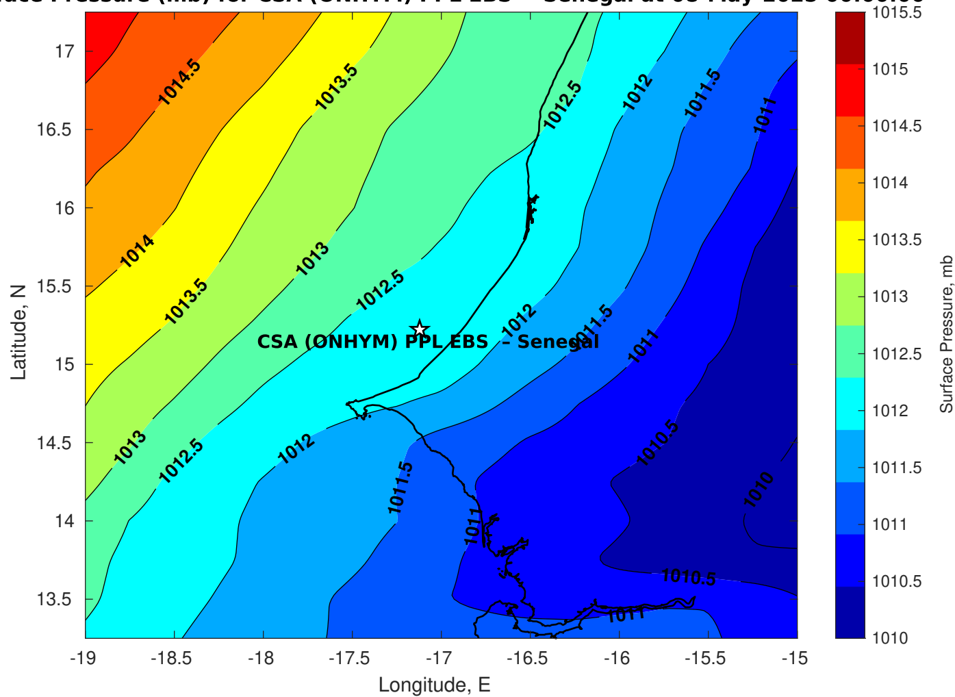
Surface Pressure (mb) for CSA (ONHYM) PPL EBS - Senegal at 08-May-2025 00:00:00
