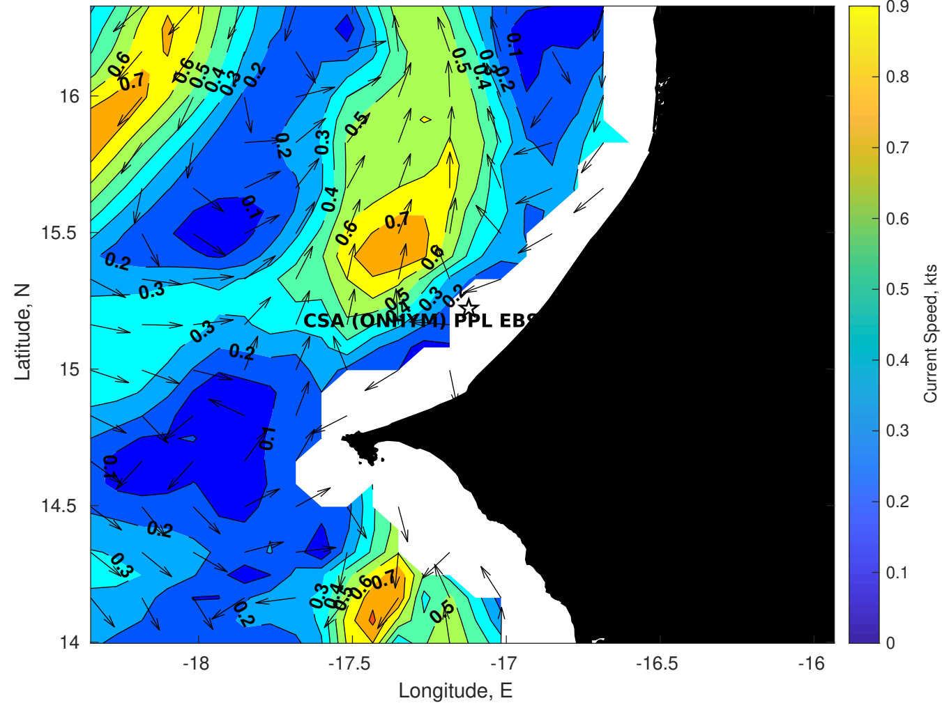
Surface Currents for CSA (ONHYM) PPL EBS - Senegal at 05-May-2025 00:00:00
