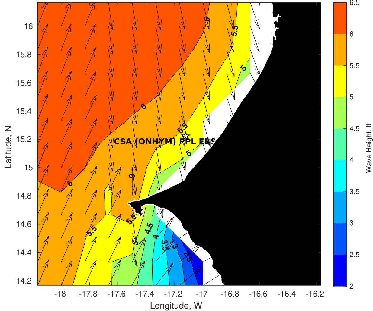
Wave Height (ft) for CSA (ONHYM) PPL EBS - Senegal at 06-May-2025 09:00:00
