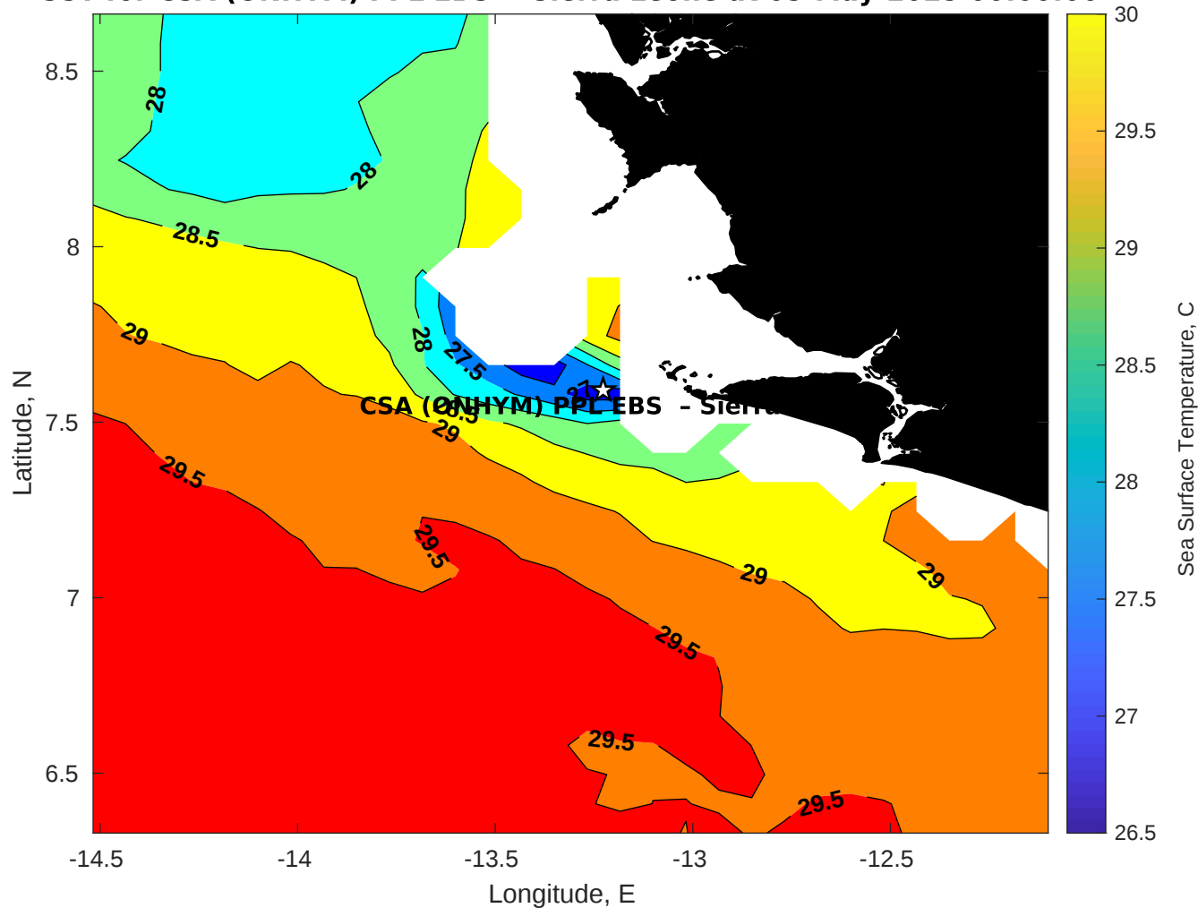
SST for CSA (ONHYM) PPL EBS - Sierra Leone at 05-May-2025 00:00:00
